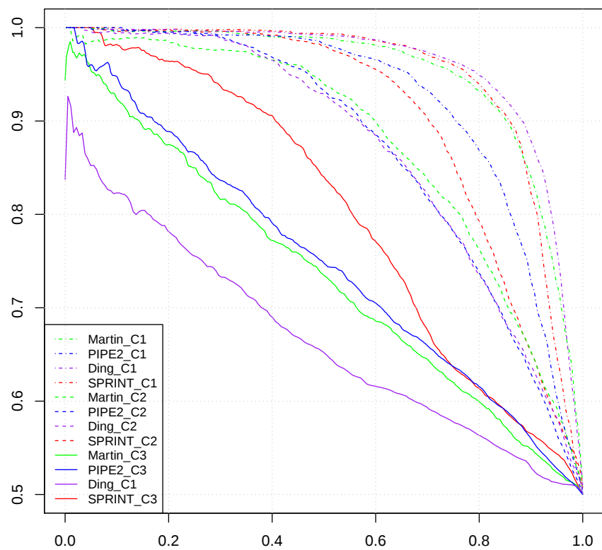
Innate_Man (C123, PR)
