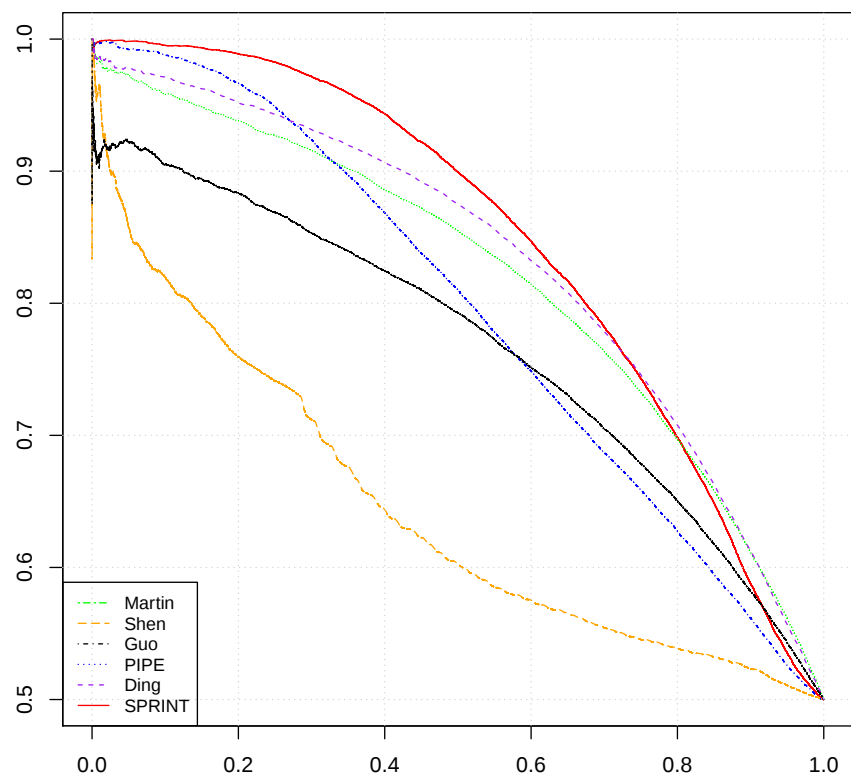
Park and Marcotte (CV, PR)
