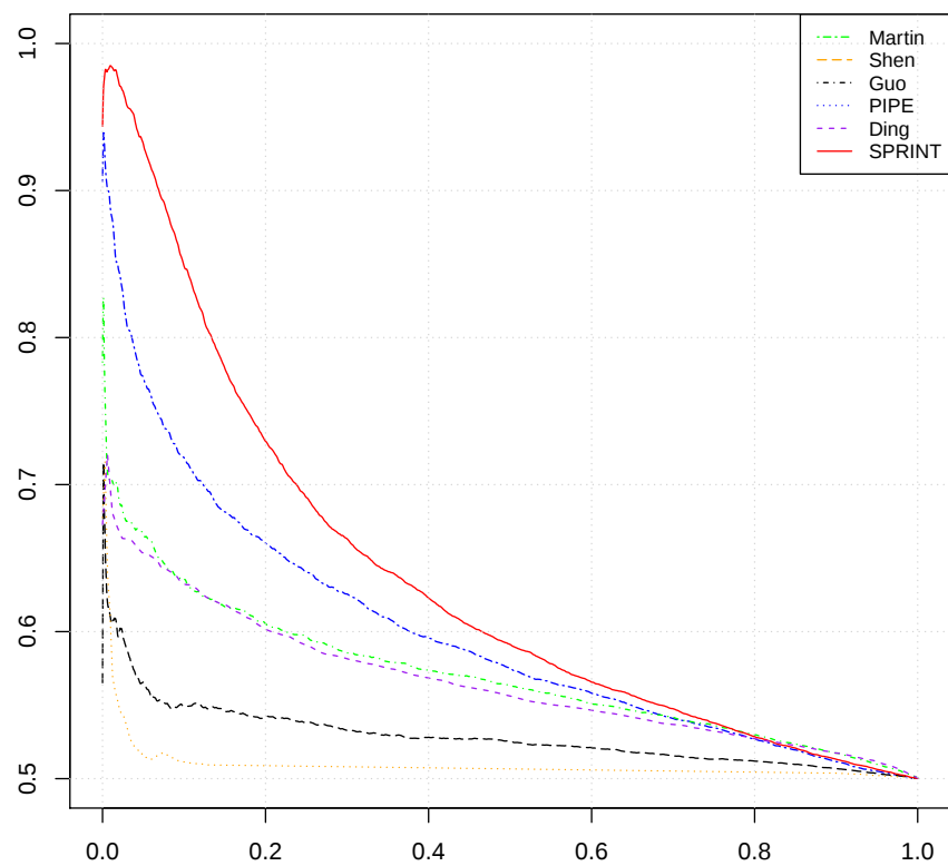
Park and Marcotte (C3, PR)
