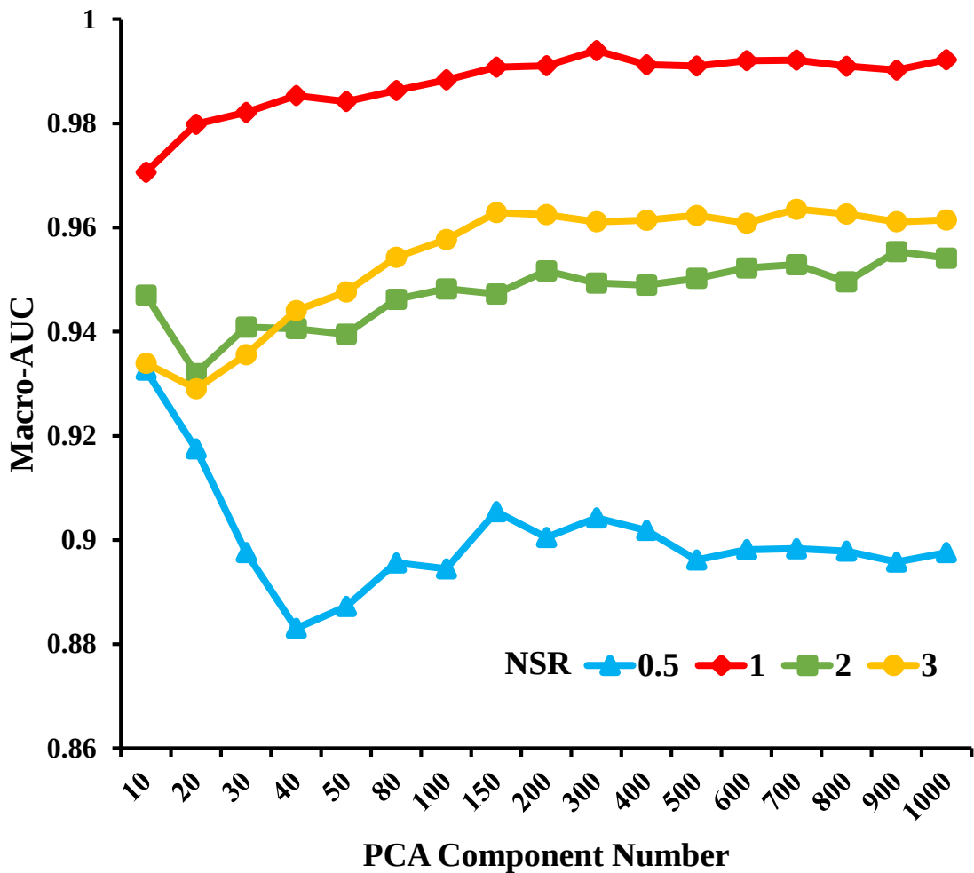
Figure S1. The macro-averaging AUCs with different PCA component number and different negative sample ratios.
