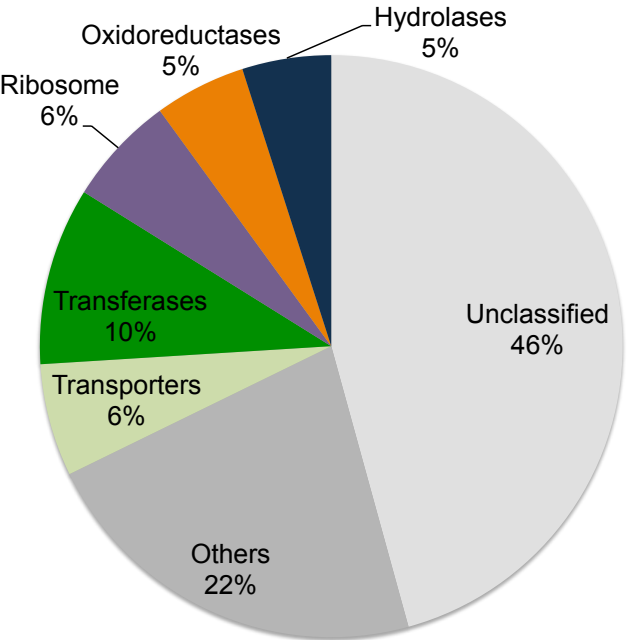
BUSCO fungi (1,439 proteins)
