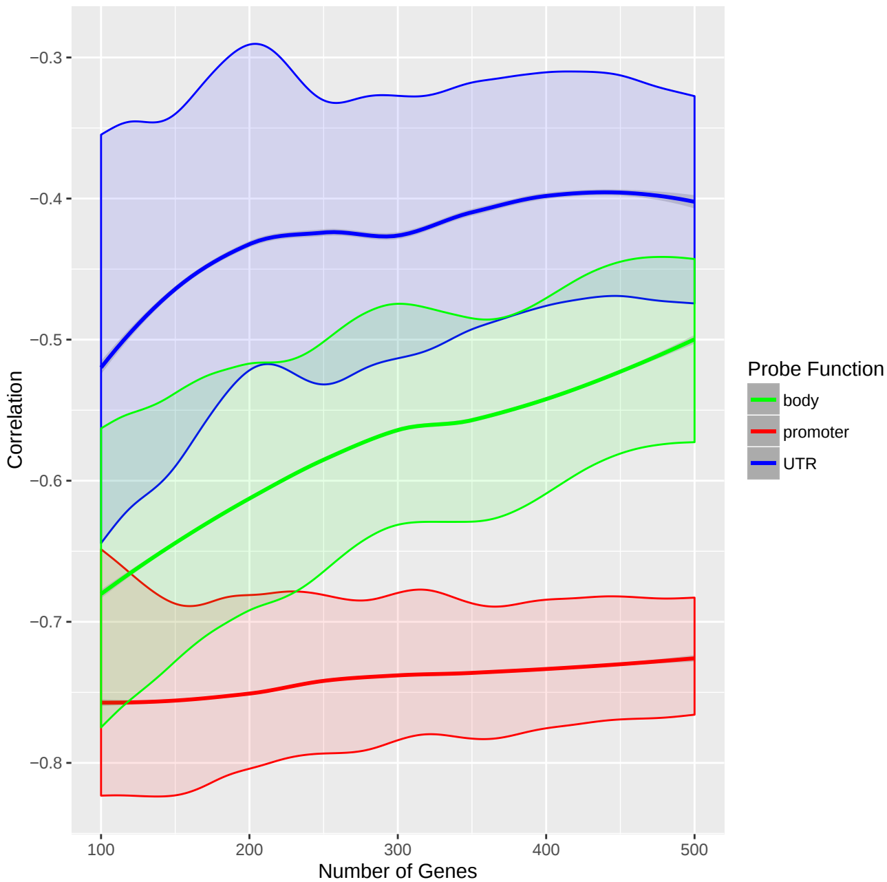
Skewness, M-value Correlation vs. Number of Included Genes in SKCM
