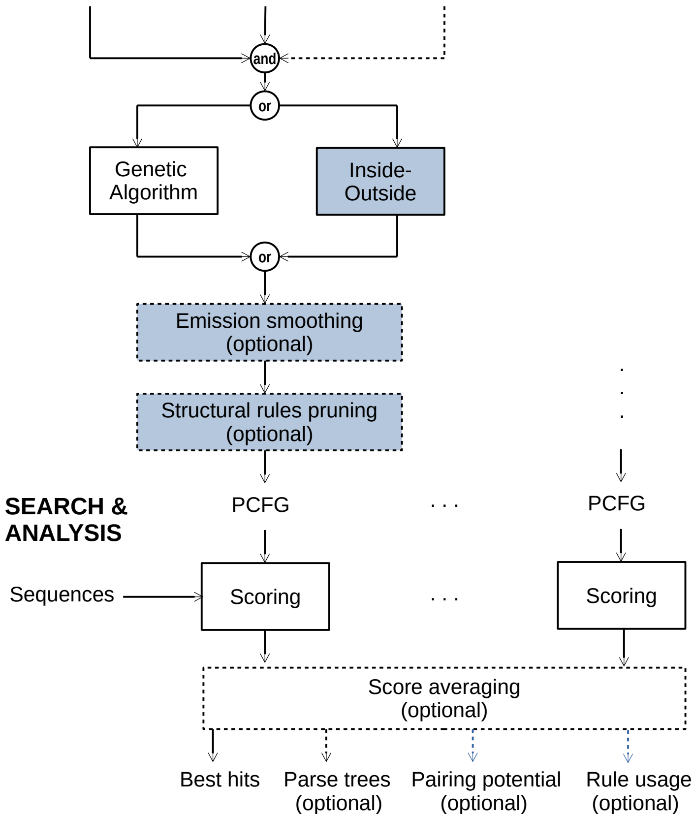
Supplementary Figure 1: The outline of the processing pipeline in the probabilistic context-free grammar-based framework for protein sequence analysis. Optional features, inputs and outputs are marked with dotted lines. Newly introduced features and outputs are marked with grey blue.
