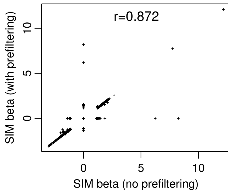
Supp Fig S1: Comparison of sparse insulation model (SIM) beta estimation with and without prefiltering of variables by lasso regression.
