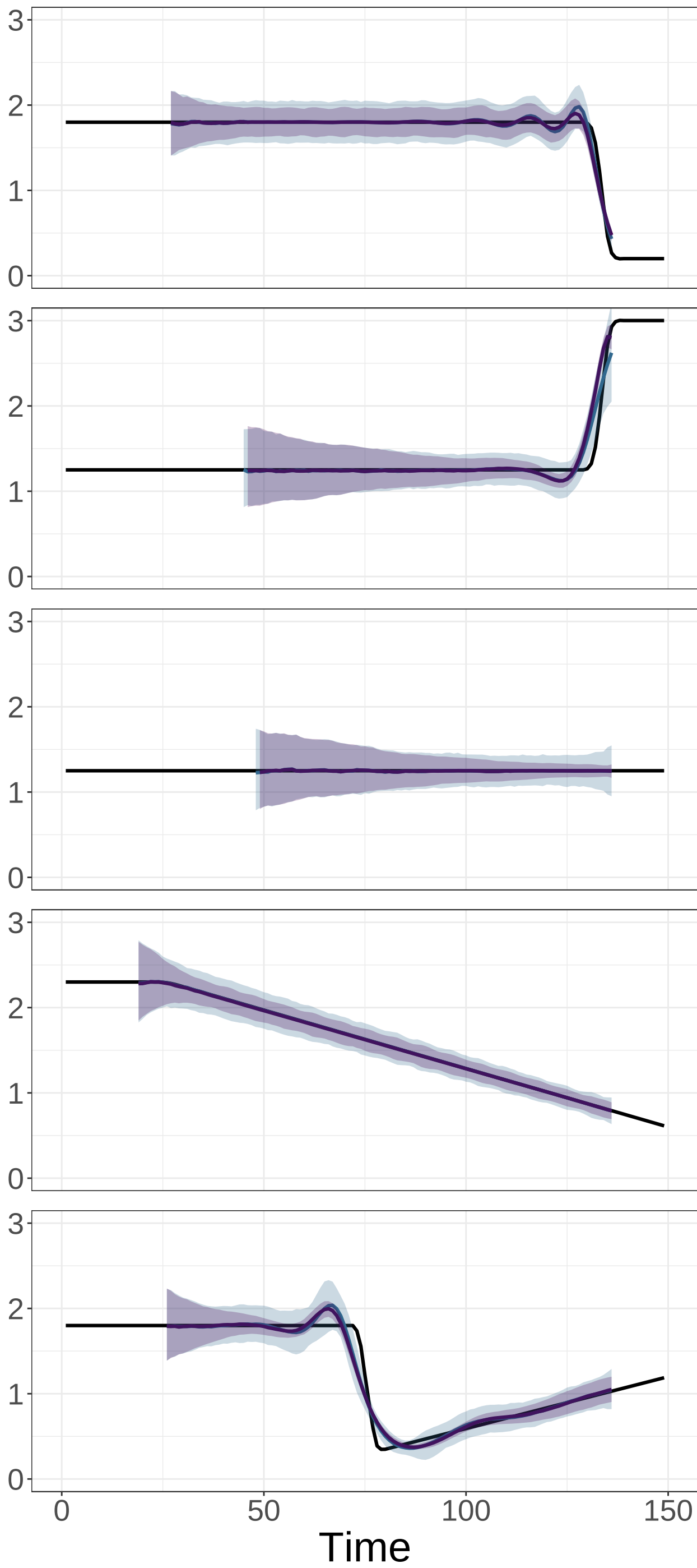
(A) Reproductive number
