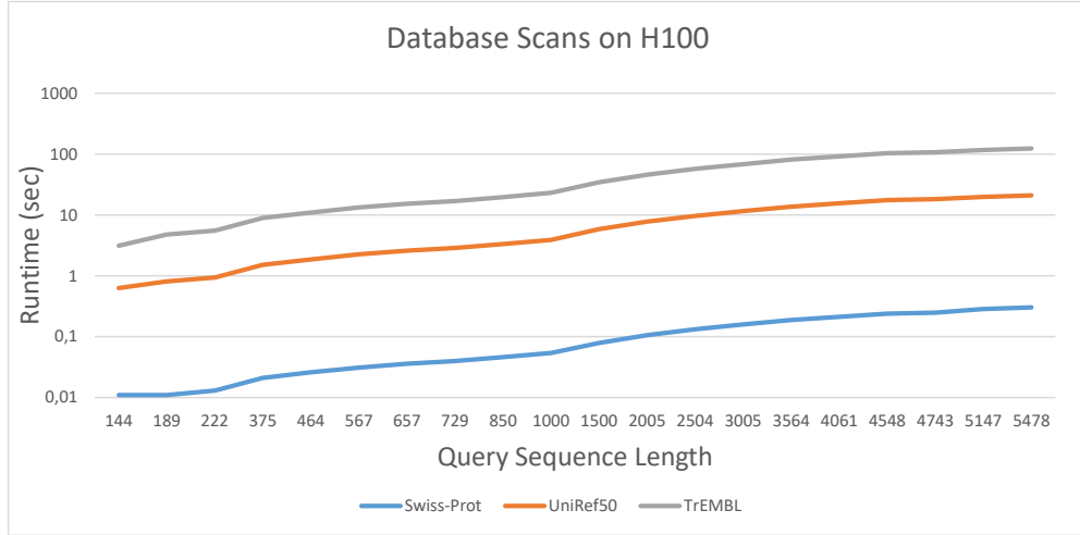
Figure 1: CUDASW++4.0 runtimes (in seconds) for scanning Swiss-Prot, UniRef50, and TrEMBL with queries of different length on H100.
