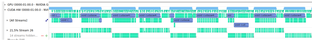
Figure 2: Screenshot of the Nsight systems profiler for execution of CUDASW++4.0 using a query of length 222 to scan a batched UniRef50 database.
