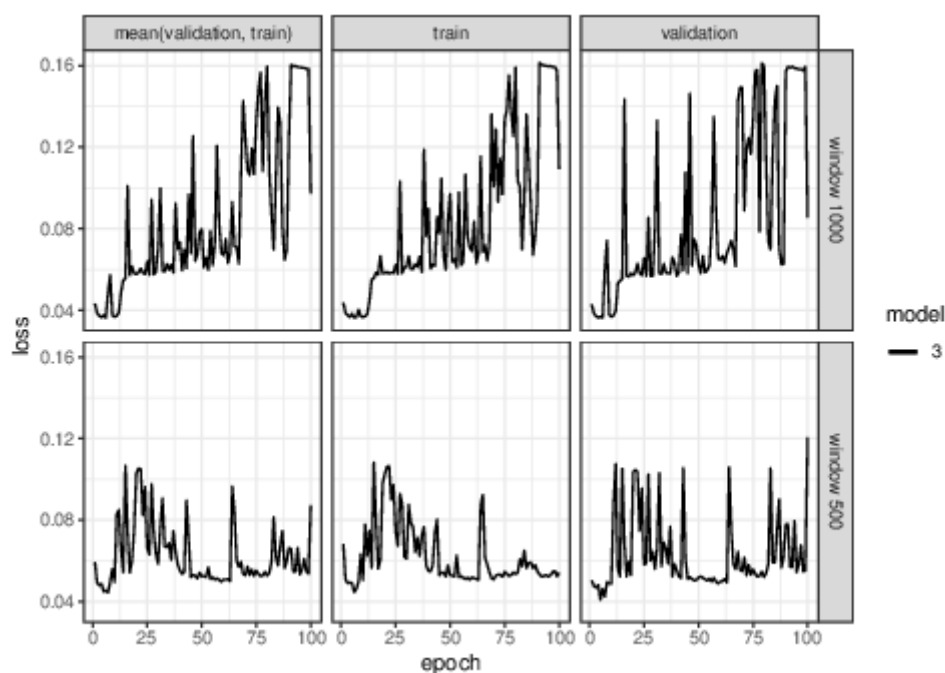
The 100 epochs train history loss of model 3 (1d CNN without batch normalization) for window 1000 and window 500 train data sets.
