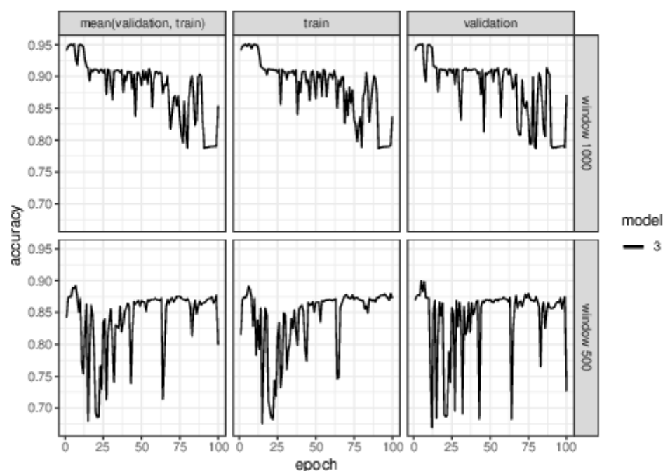
The 100 epochs train history accuracy of model 3 (1d CNN without batch normalization) for window 1000 and window 500 train data sets.
