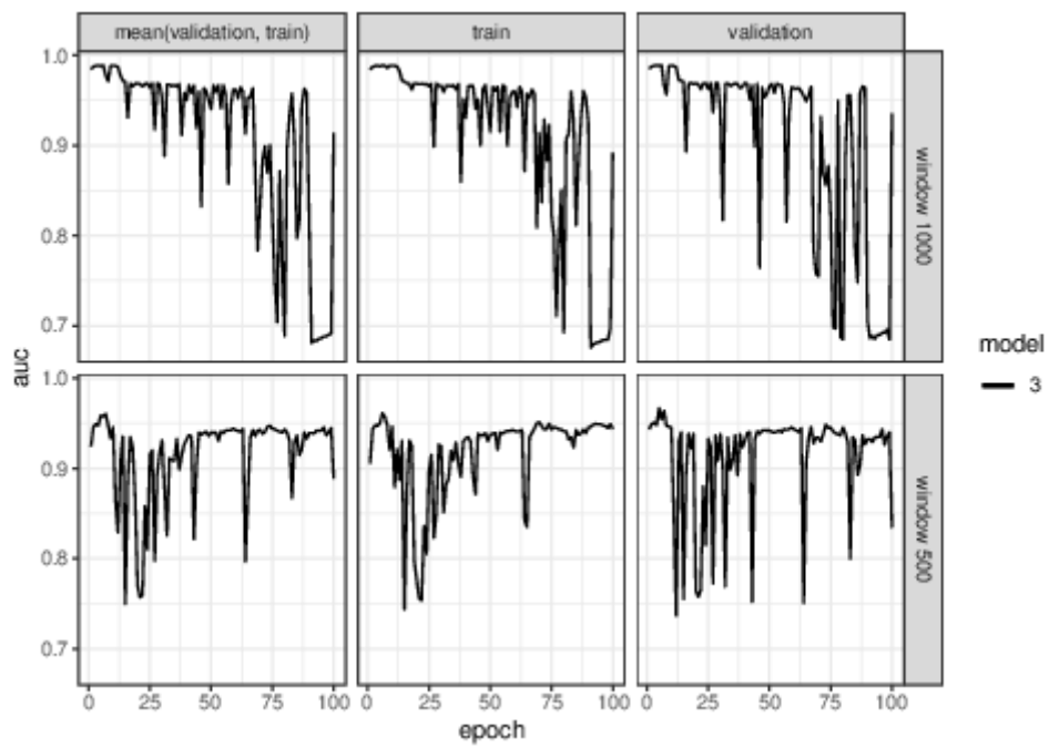
The 100 epochs train history AUC of model 3 (1d CNN without batch normalization) for window 1000 and window 500 train data sets.
