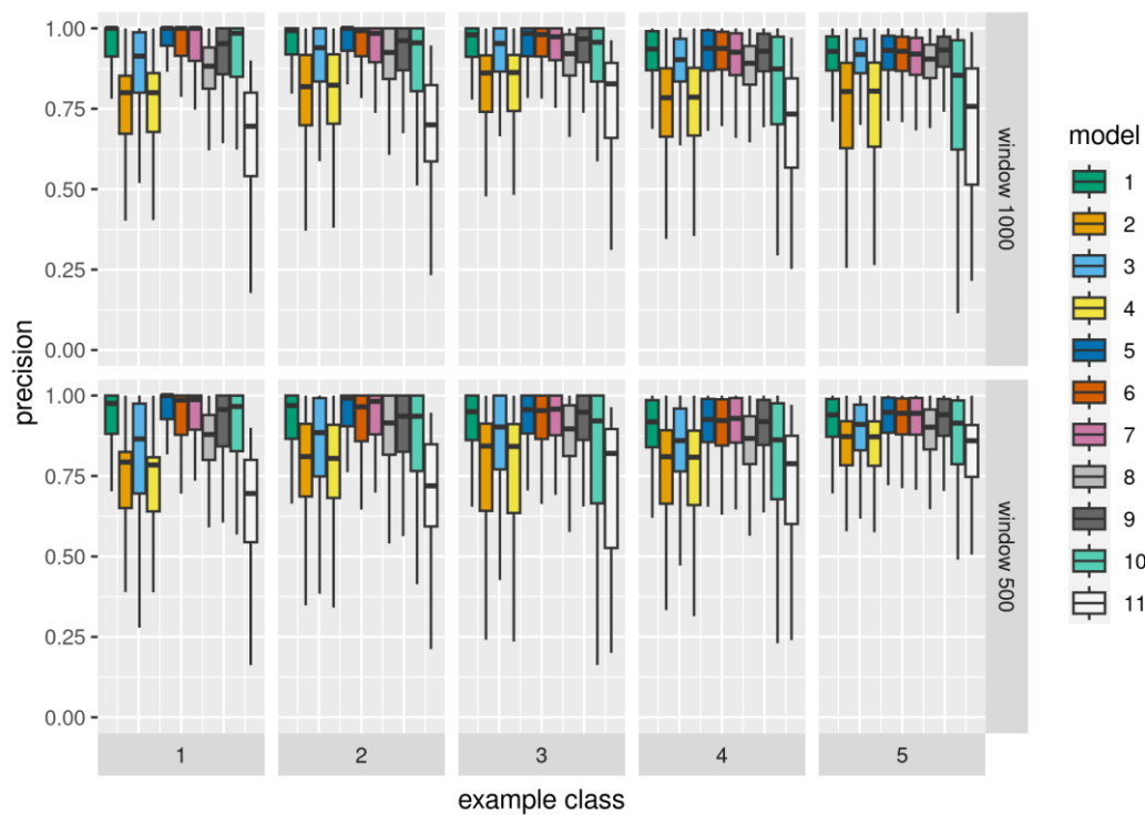
Distribution of the precision metric for the 5 train classes based on the 1M individual predictions of evaluation data set
