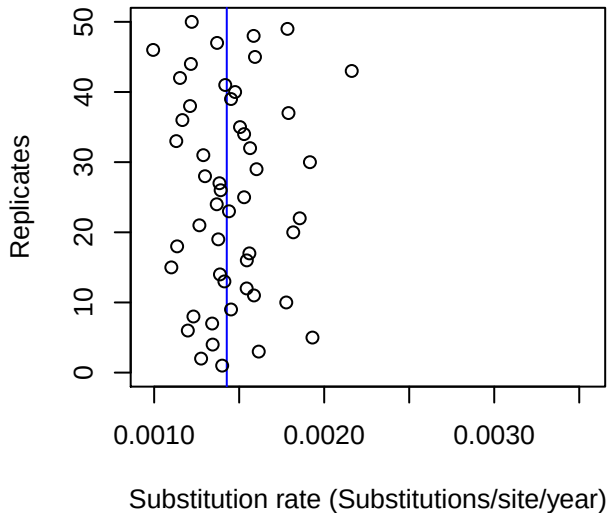
(a) Linear regression
