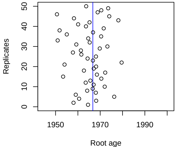
(b) Linear regression
