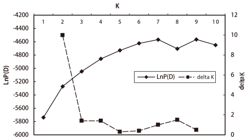
Figure S2 Results of Bayesian clustering analysis performed in STRUCTURE. For each K tested, the Ln P (D) equals the mean of the estimated log of the probability of the data across 10 different runs, while the \Delta K was determined by the second order rate of change of these log likelihoods.
