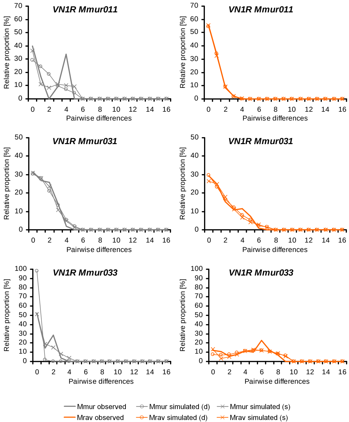
Additional file 2: Observed and simulated mismatch distributions of M. murinus (Mmur, left side, grey) and M. ravelobensis (Mrav, right side, orange); simulated (d) = simulated after demographic expansion model (line with circles), simulated (s) = simulated after spatial expansion model (line with crosses); (continues on next pages)
