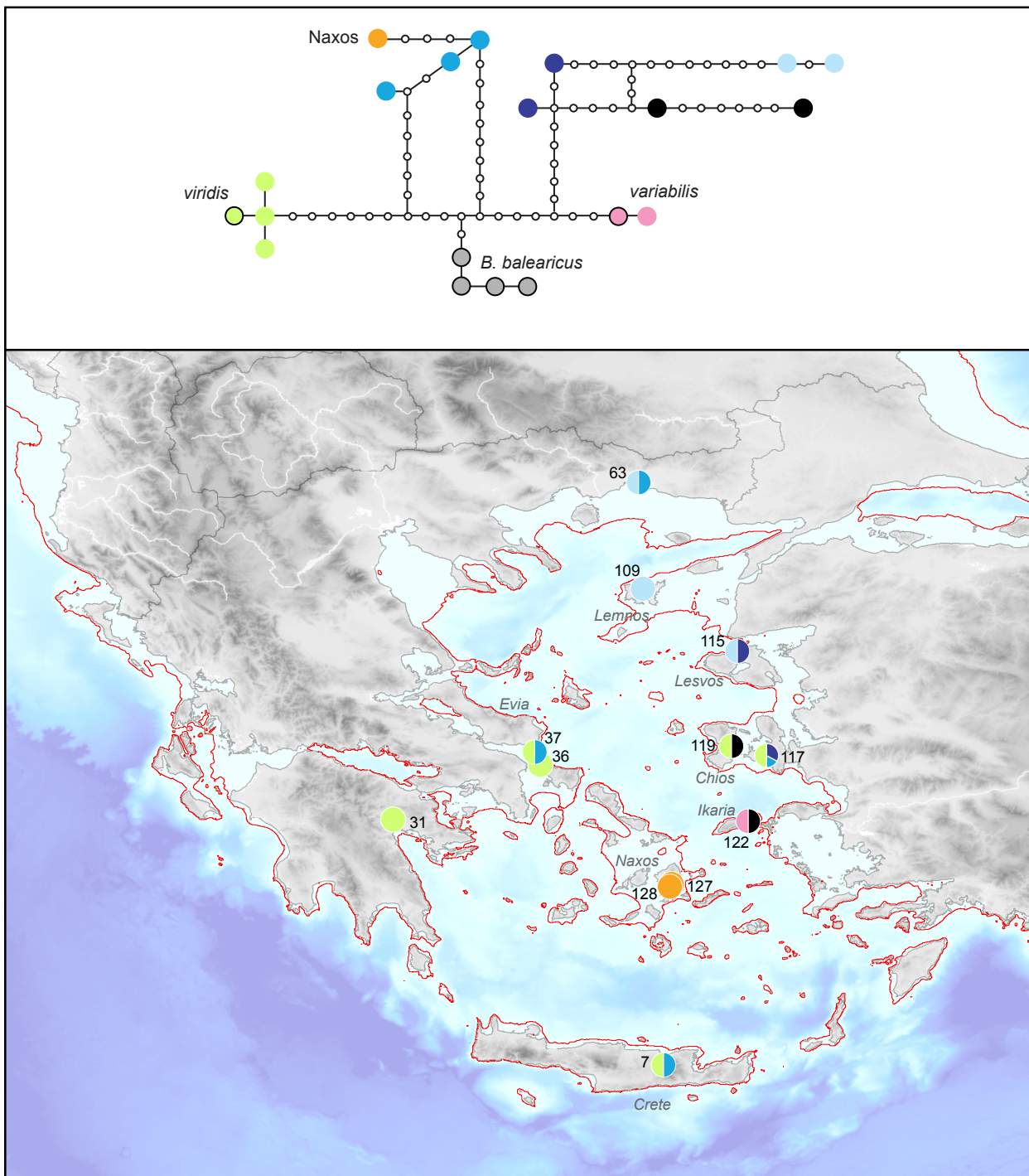
Fig. S1: Haplotype network of the tropo intron marker, and distribution of the main haplogroups. Circles haplotypes show reference sequences for each species. Colors were tentatively attributed to the main nuclear clusters inferred from microsatellites.
