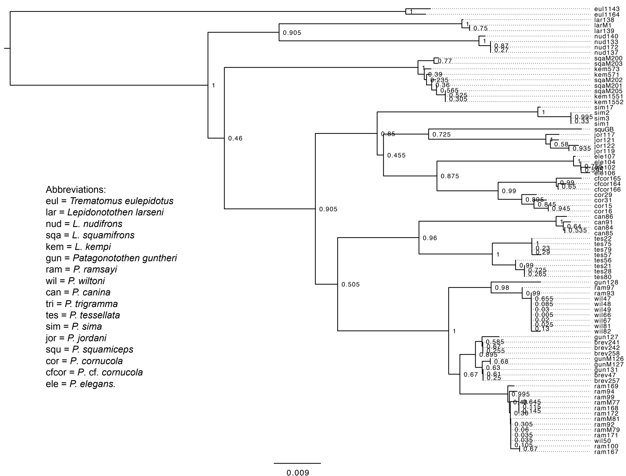
Additional file 6. Neighbour Joining tree based on COI sequences of 620 bp. Node labels represent bootstrap support values as obtained with MEGA 6.06.
