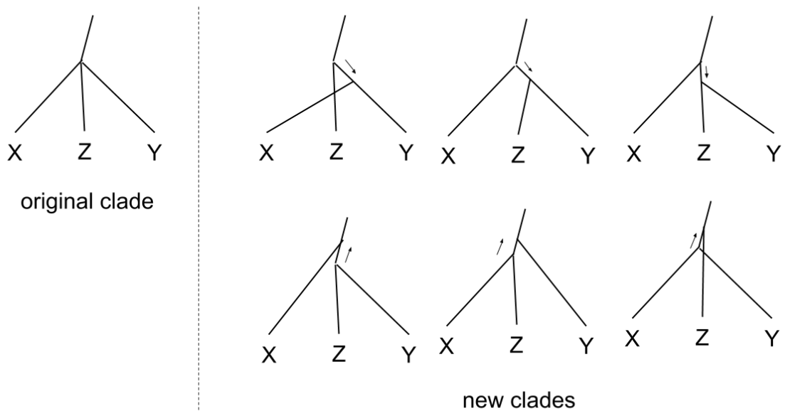
Supplementary Figure S2. Illustration of possible local moves that split an internal node into two. For an internal node that has more than two children, possible moves comprise moving the node upwards or downwards by one time-step (not shown), and also moving one of its downstream branches upwards or downwards by one time-step and splitting the internal node into two (all 6 possible moves that split an internal node with 3 children are shown).
