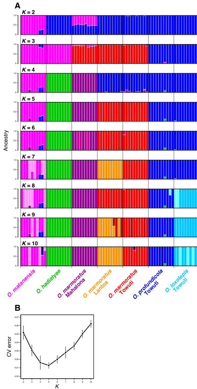
Fig. S3 (A) ADMIXTURE results showing K = 2 – 10 genetic clusters based on 4,193 SNPs from the seven populations in the Malili Lake system. (B) Cross-validation errors (mean \pm standard deviation) for each K , based on 10 independent ADMIXTURE runs
