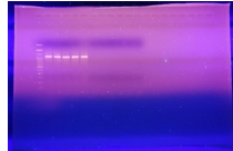
Figure 3 B Contig 1
