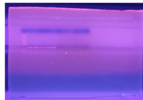
Figure 3 A Contig 4
