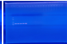
Figure 3 A Actin
