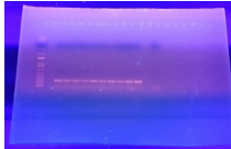
Figure 3 B Contig 3
