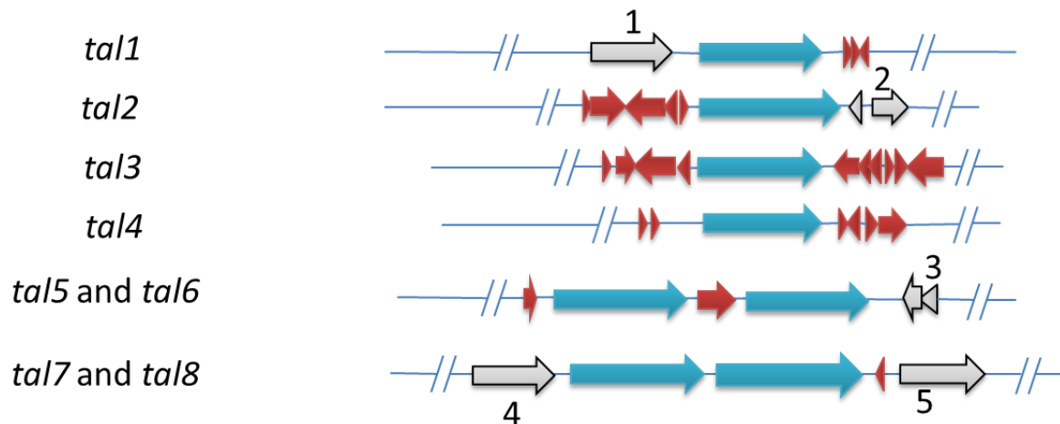
Figure S9. Most TAL effector genes are flanked by transposon elements. The blue arrows indicate the TAL effector genes and the dark red arrows show the transposase genes; the gray arrows indicate other genes. The genes are listed as following: 1, RpoD , encoding RNA polymerase subunit sigma-70; 2, Hypothetical genes; 3, Acetyltransferase and hypothetical genes; 4, Type III effector gene xopL ; 5, vgrG , encoding type IV secretion protein.
