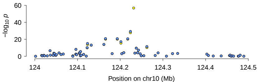
B: ARMS2
