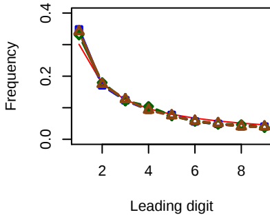
Paired end reads
