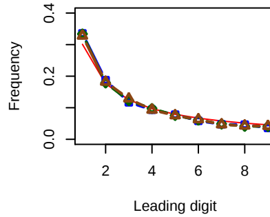
Single end reads(SE)
