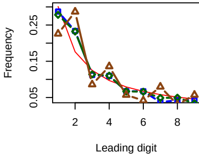
Paired end reads
