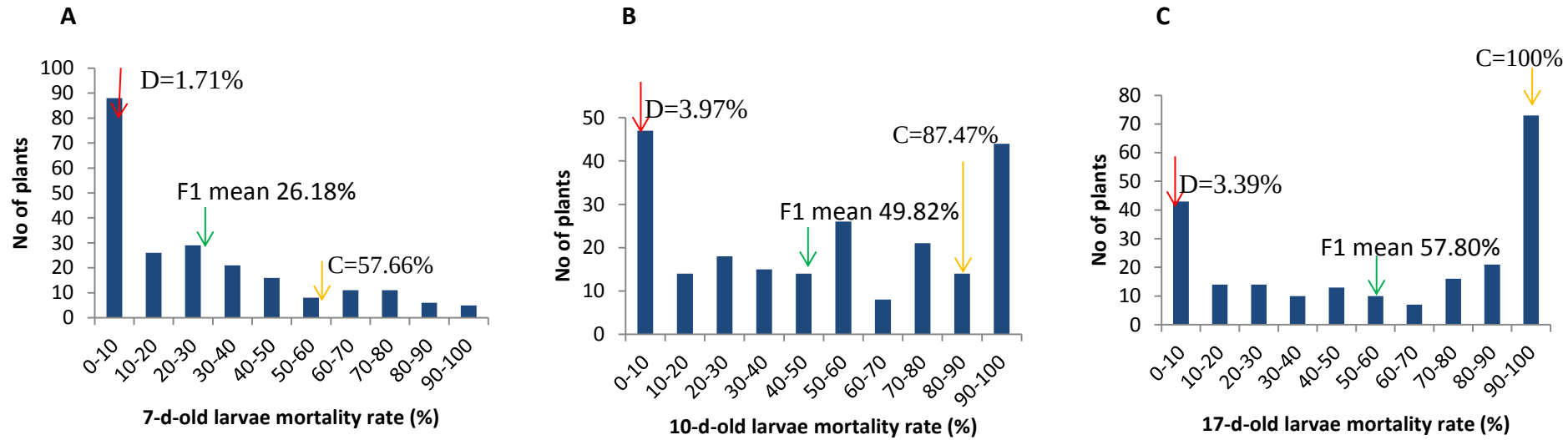
Figure S4 The frequency distribution of the mortality rate of larvae fed leaf tissue from each individual of the mapping population. D: cultivar ‘Diamond’ (susceptible); C: cultivar ‘Cavalier’ (resistant).
