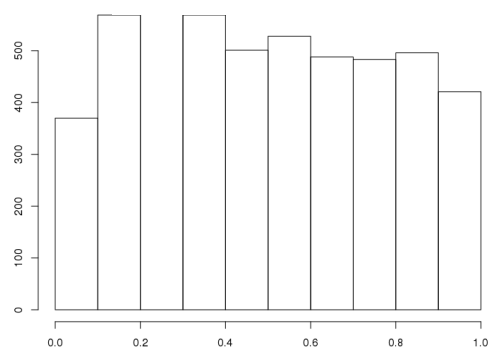
GUCY1A3
