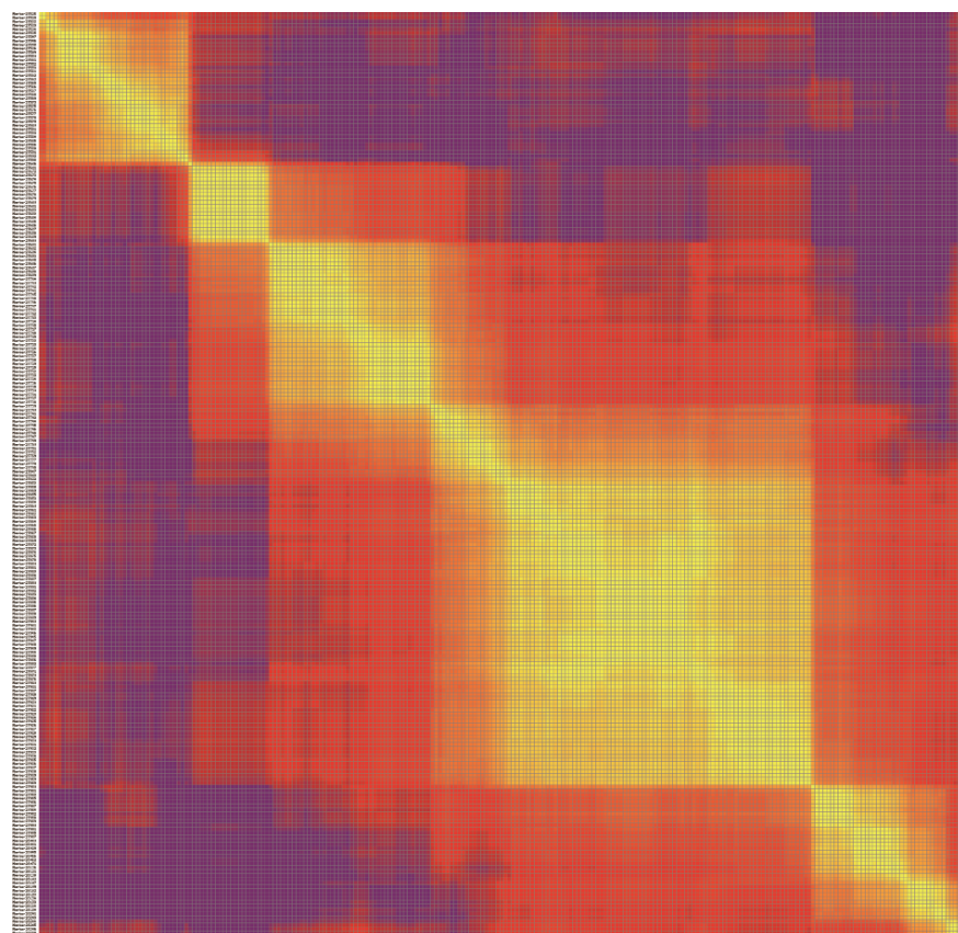
Chromosome D5
