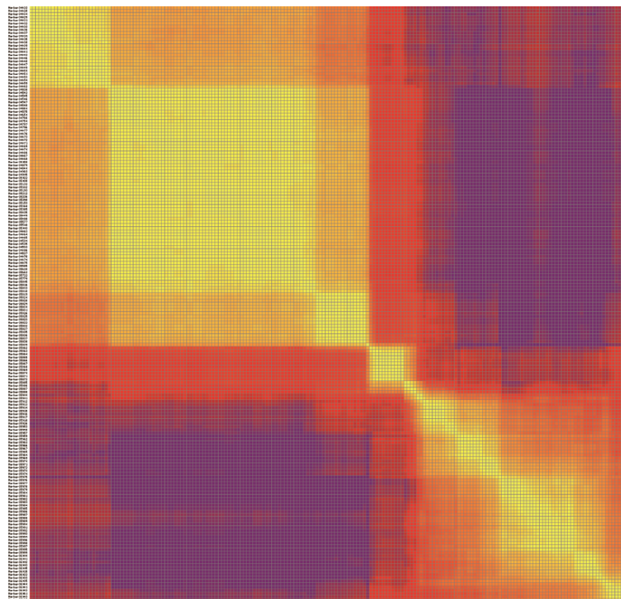
Chromosome D9
