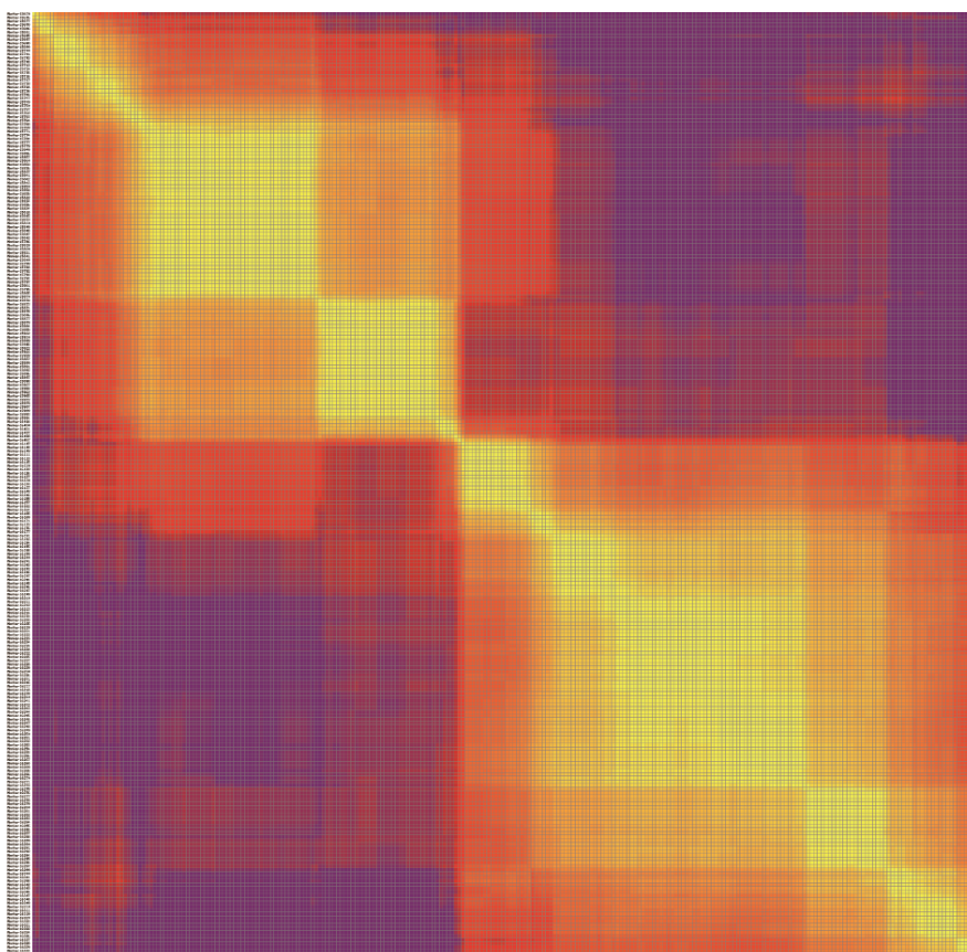
Chromosome A10
