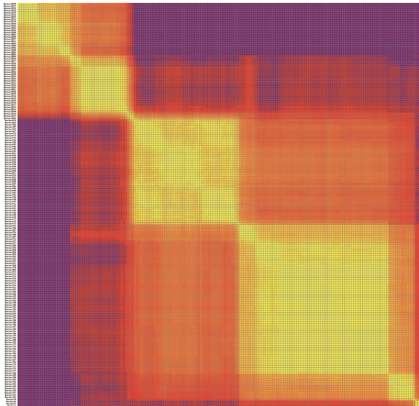
Chromosome A1
