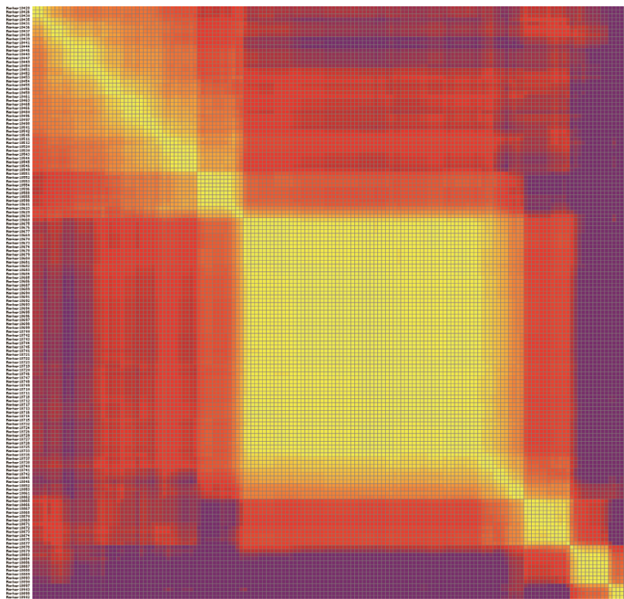
Chromosome A12
