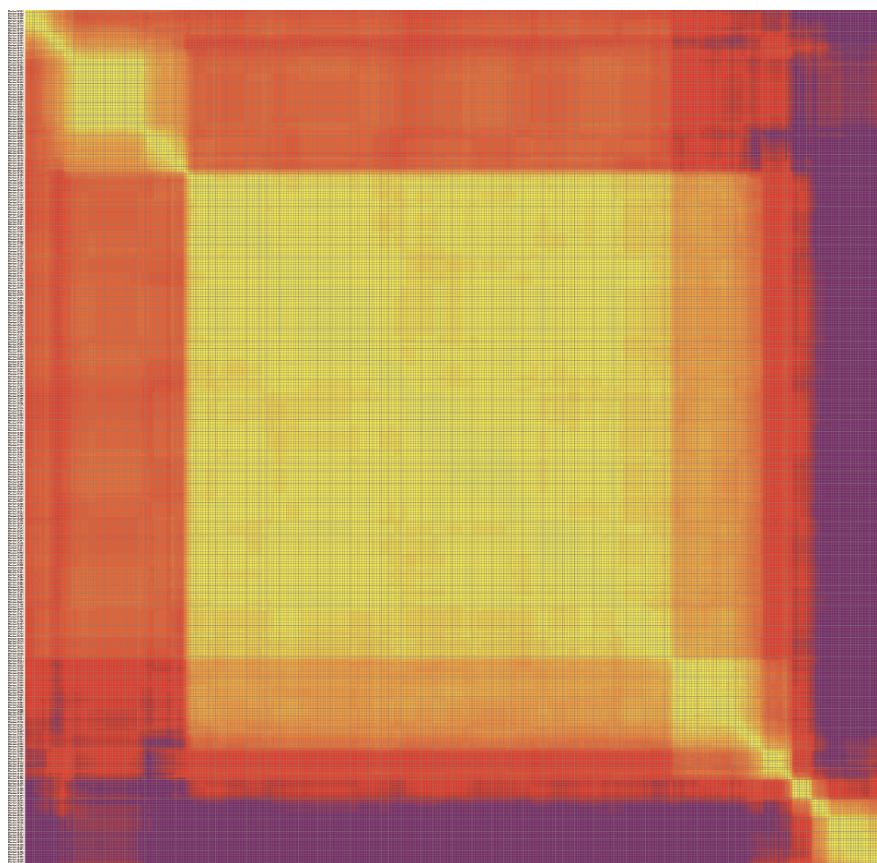
Chromosome A11
