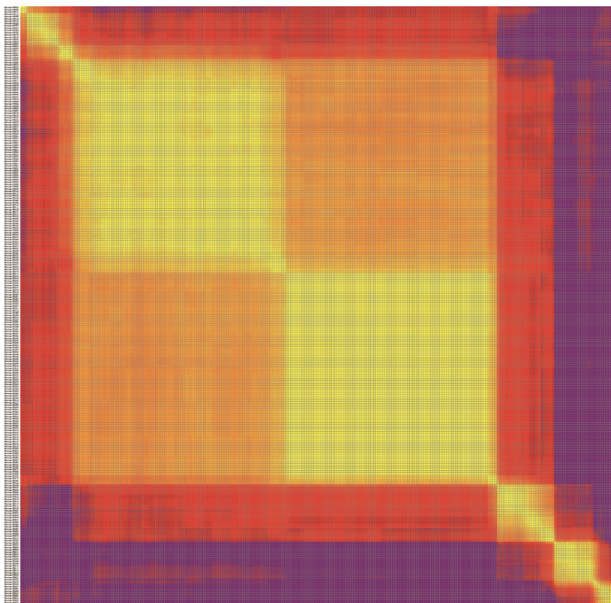
Chromosome A9
