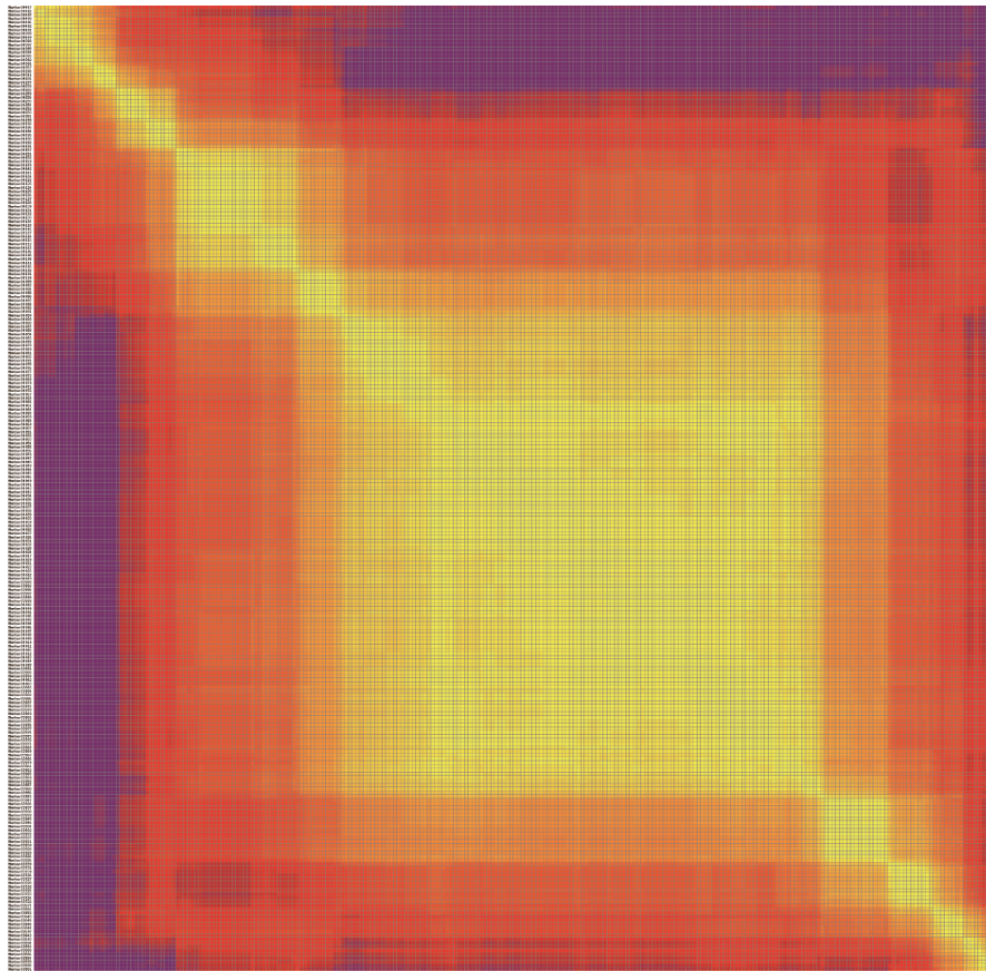
Chromosome D8
