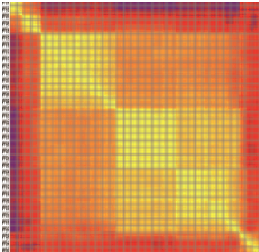
Chromosome A2
