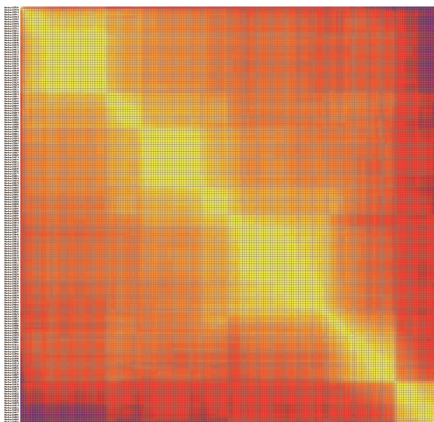
Chromosome D3
