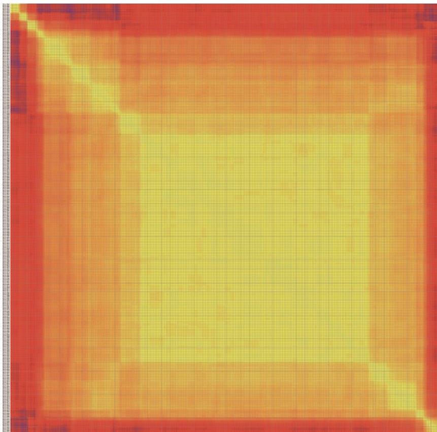
Chromosome A8
