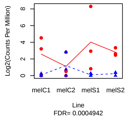
CG44014 ( FBgn0264776 )
