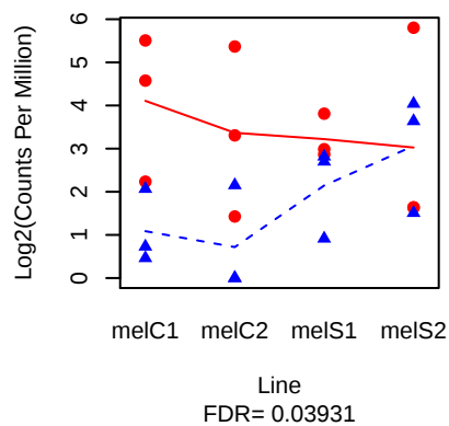
NA ( FBgn0053271 )
