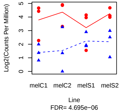
CG4716 ( FBgn0033820 )
