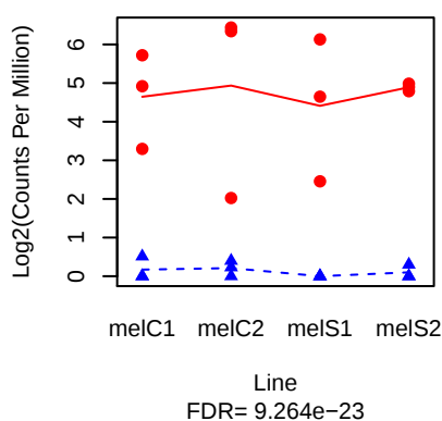
CG43085 ( FBgn0262531 )
