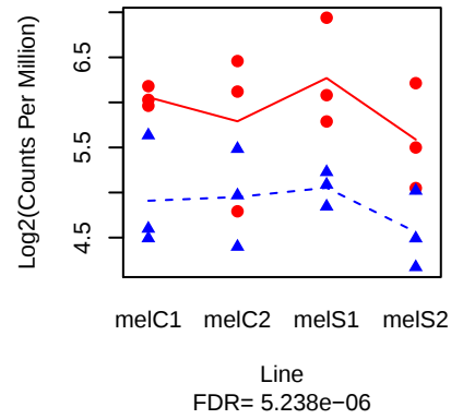
IM2 ( FBgn0025583 )
