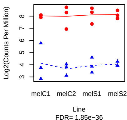
CG44475 ( FBgn0265668 )
