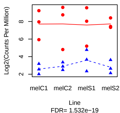
lectin-24A ( FBgn0040104 )
