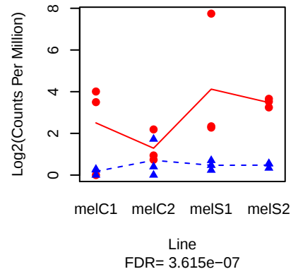
CG13559 ( FBgn0034870 )
