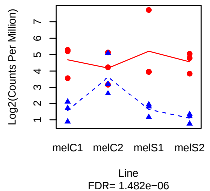
CG18067 ( FBgn0034512 )
