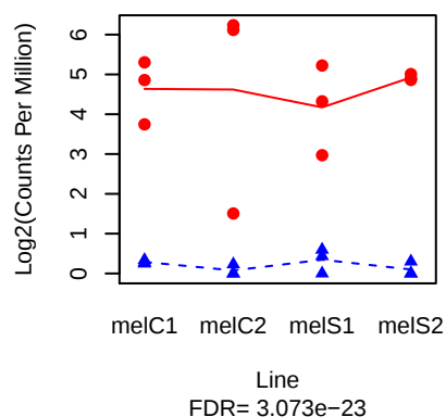
Tep1 ( FBgn0041183 )
