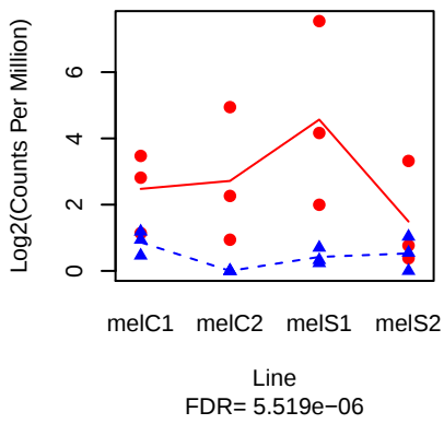
IM23 ( FBgn0034328 )
