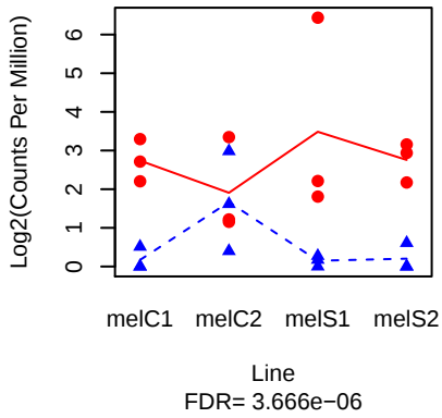
AttA ( FBgn0012042 )
