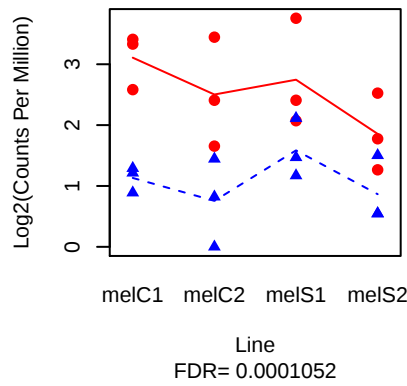
AttB ( FBgn0041581 )
