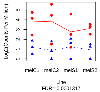
CG15067 ( FBgn0034331 )
