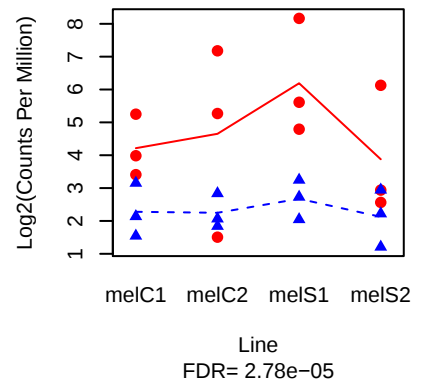
NA ( FBgn0262588 )
