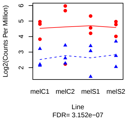
CG33226 ( FBgn0069056 )
