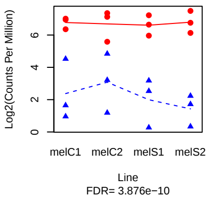
CG34436 ( FBgn0085465 )
