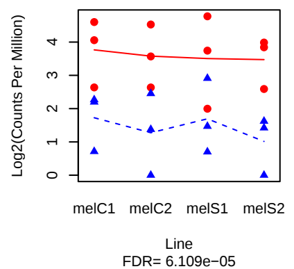
NA ( FBgn0262588 )
