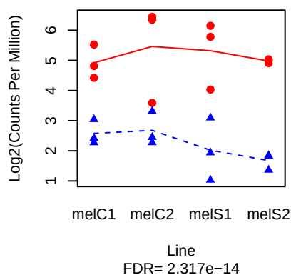
CG33459 ( FBgn0053459 )
