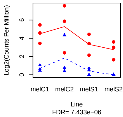
edin ( FBgn0052185 )
