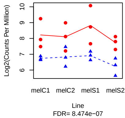
NA ( FBgn0040736 )
