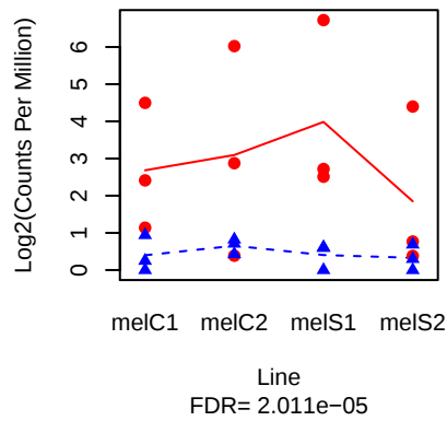
Sp7 ( FBgn0037515 )
