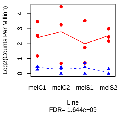
CG34436 ( FBgn0085465 )
