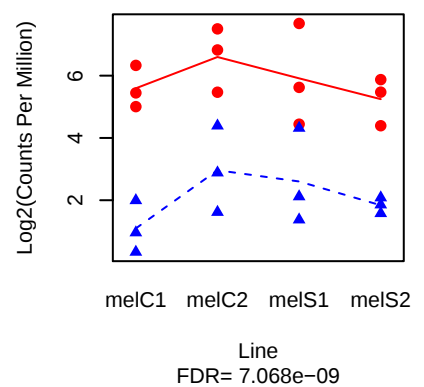
NA ( FBgn0262607 )
