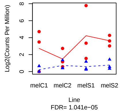
PGRP-SB1 ( FBgn0043578 )
