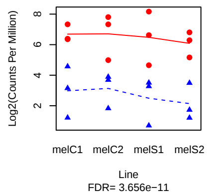
CG4793 ( FBgn0028514 )
