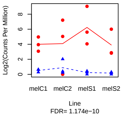
CG43153 ( FBgn0262683 )
