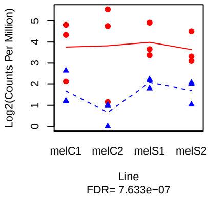
Dro ( FBgn0010388 )
