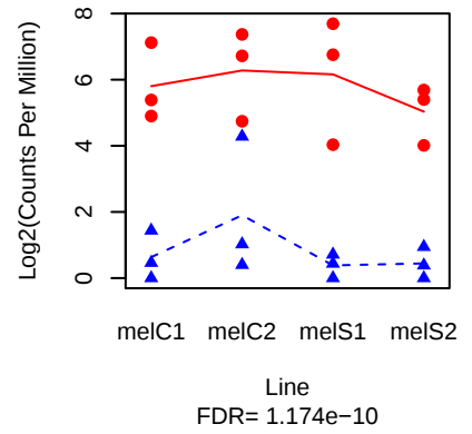
Spn88Eb ( FBgn0038299 )
