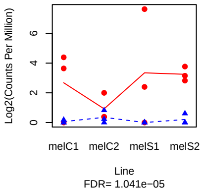
CG11313 ( FBgn0039798 )
