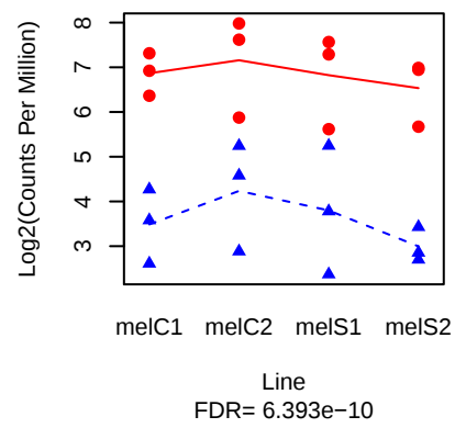
NA ( FBgn0262607 )
