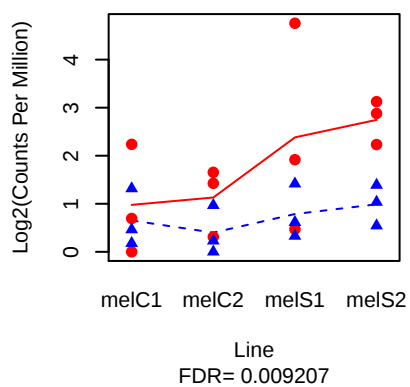
Spn43Ad ( FBgn0044011 )
