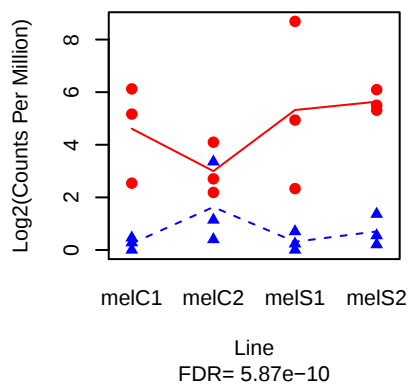
SPH93 ( FBgn0032638 )
