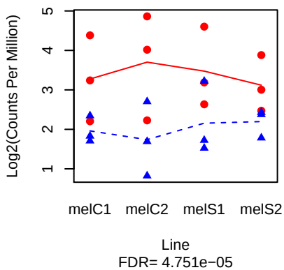
CG11313 ( FBgn0039798 )
