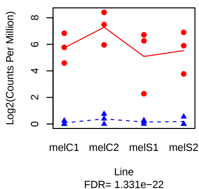
CG18557 ( FBgn0031470 )
