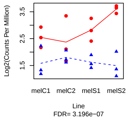
Tep2 ( FBgn0041182 )
