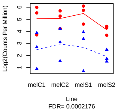
CG9616 ( FBgn0038214 )
