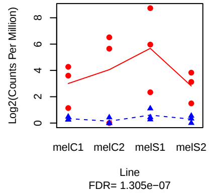
GNBP-like3 ( FBgn0034511 )
