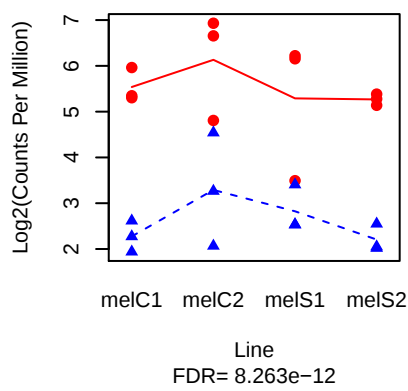
CG30091 ( FBgn0050091 )
