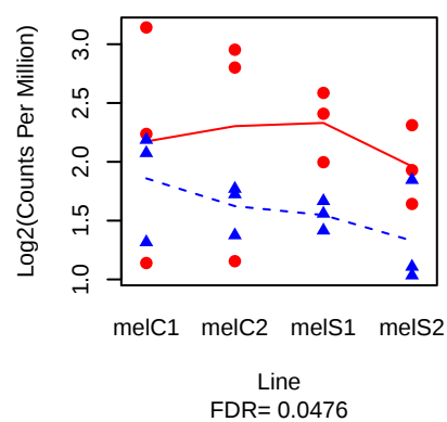
Cyp4ac3 ( FBgn0031695 )
