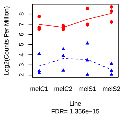
CG18563 ( FBgn0032639 )
