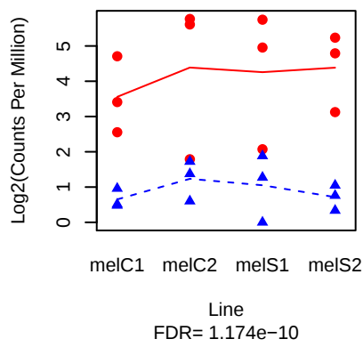
IM1 ( FBgn0034329 )
