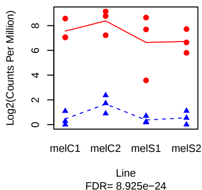
TotC ( FBgn0044812 )
