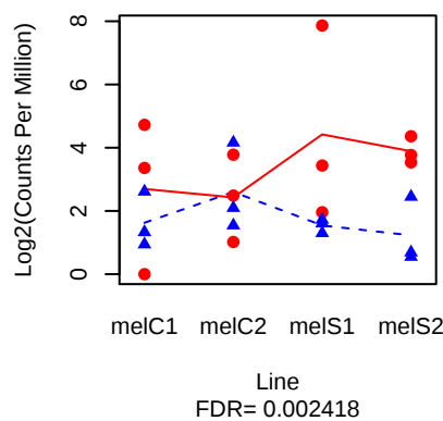
IM4 ( FBgn0040653 )
