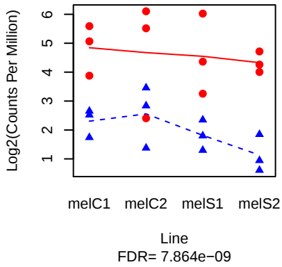
CG30414 ( FBgn0050414 )
