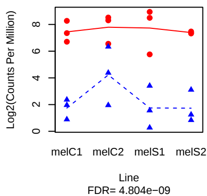
SPH93 ( FBgn0032638 )
