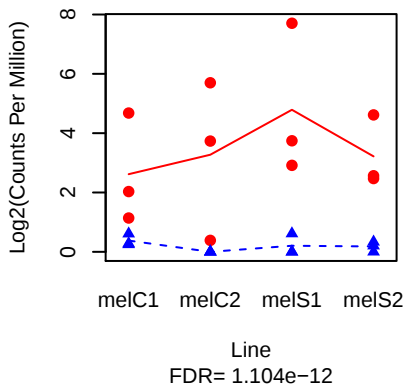
DptB ( FBgn0034407 )
