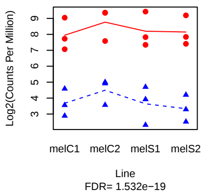
CG3117 ( FBgn0031471 )
