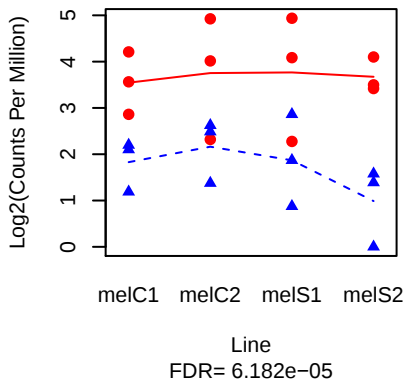
Sid ( FBgn0039593 )
