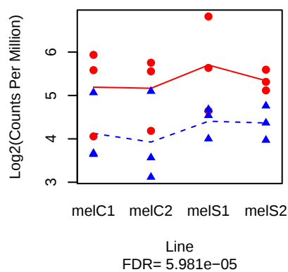
Sp7 ( FBgn0037515 )
