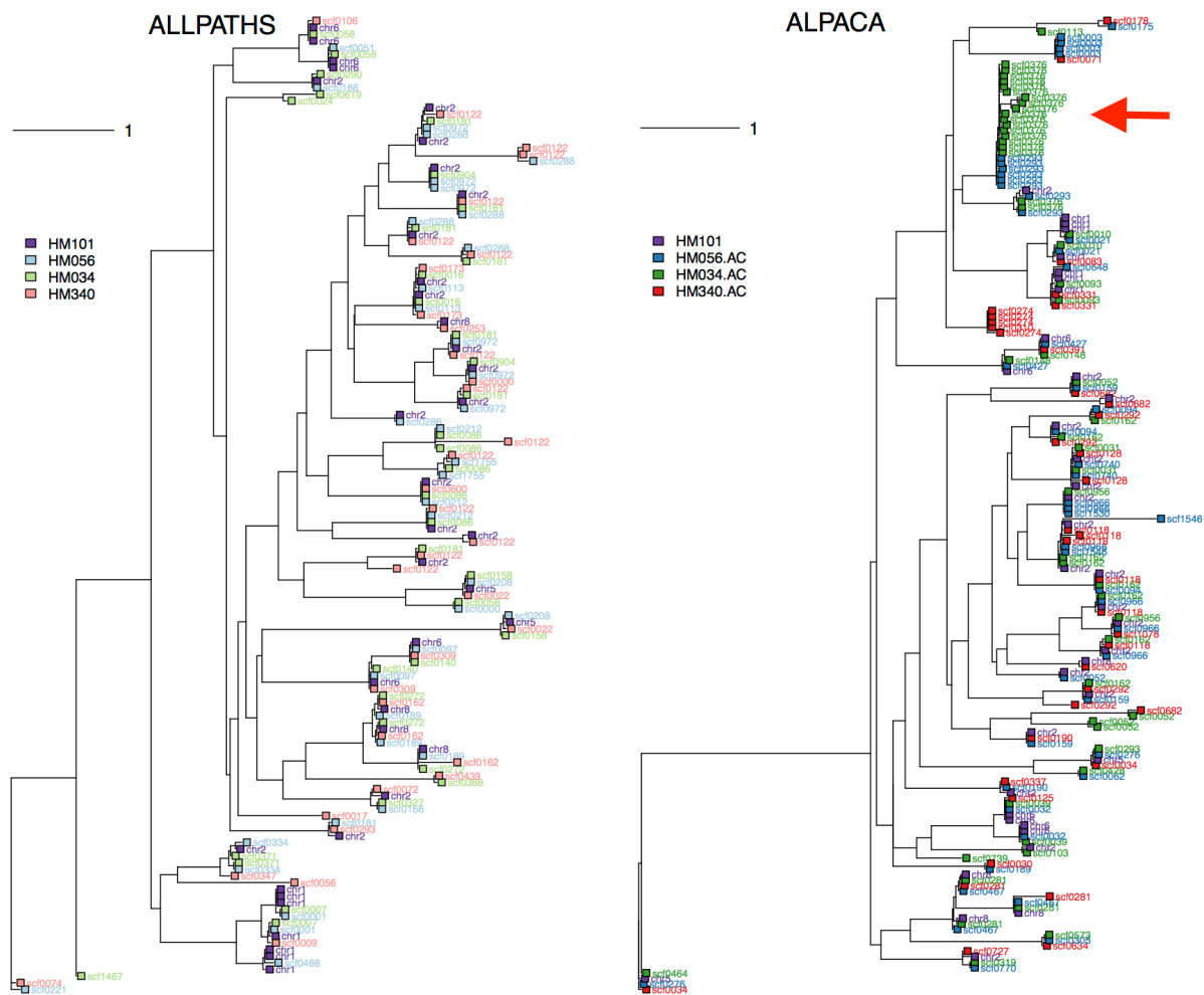
Supplemental Figure S3. Phylogeny reconstruction of the CRP0355 subfamily of the CRP gene family across four accessions of Medicago truncatula based on Mt4.0 reference assembly and three ALLPATHS assemblies (left) or three Alpaca assemblies (right). The Alpaca assembly contains accession-specific gene family expansions absent from the ALLPATHS assembly. A red arrow highlights the largest accession specific expansion.
