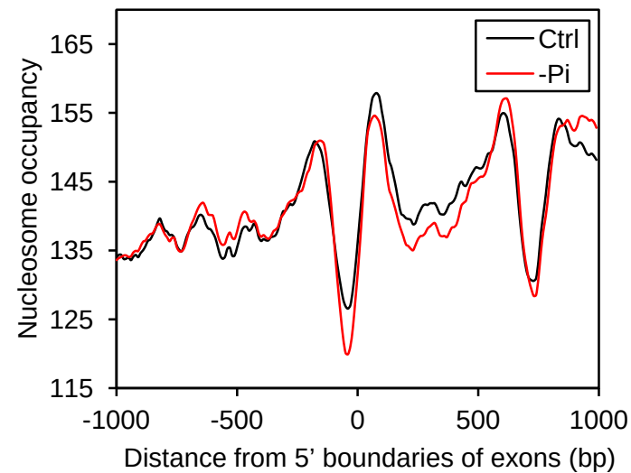
Figure S5 Changes in nucleosome occupancy at the exons of rice genes in response to phosphate starvation. MNase-seq density of exons grouped according to their length: (A) 170–240 bp; (B) 315–350 bp; (C) 480–550 bp (D) 645–715 bp under control and -Pi conditions. Plots are centered at the 5' boundaries of the exons.
