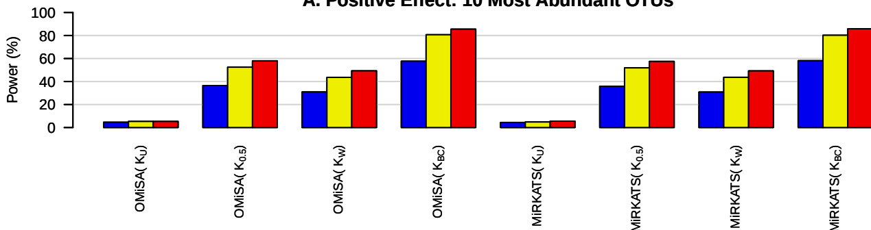
B. Positive Effect: 10 Random OTUs
