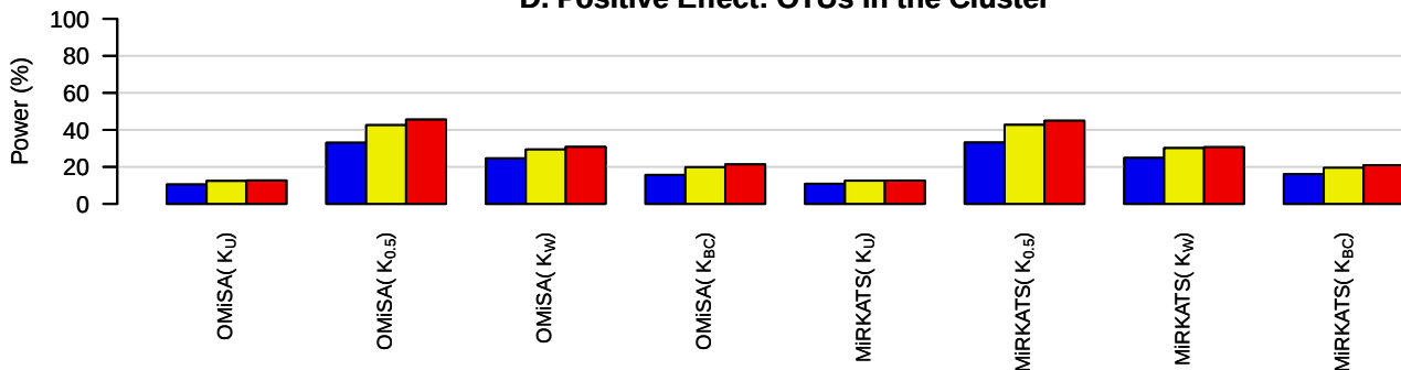
D. Positive Effect: OTUs in the Cluster
