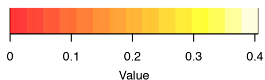
gower distance score
