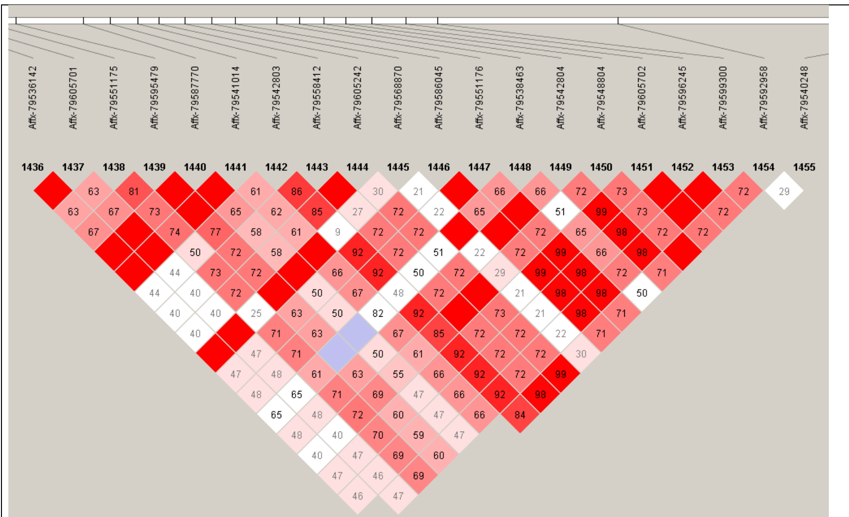
Haploview – Chr21– (59937376-60937376)
