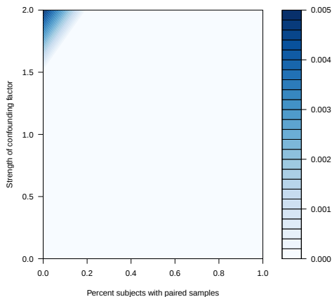
SD power with 500 total samples
