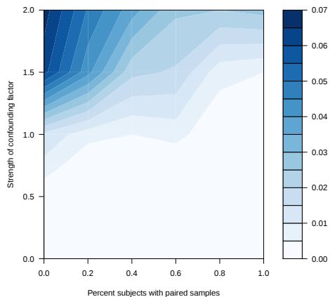
SD power with 200 total samples
