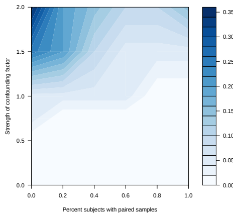
Range power with 200 total samples
