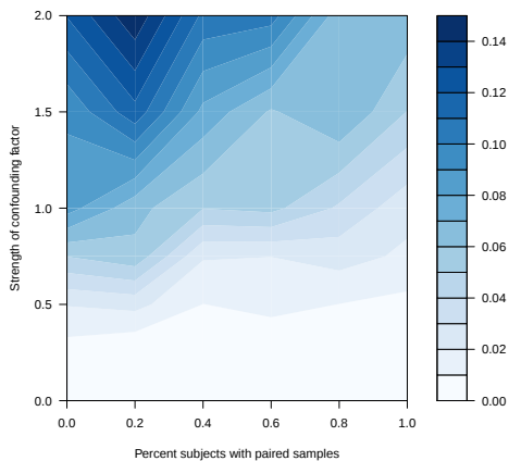
SD power with 100 total samples
