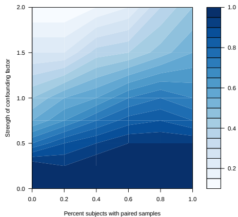
Median power with 50 total samples
