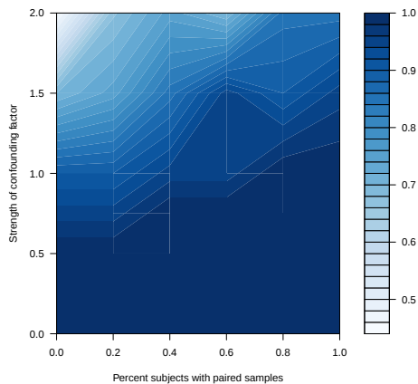
Median power with 100 total samples
