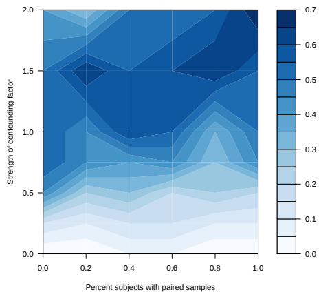
Range power with 50 total samples
