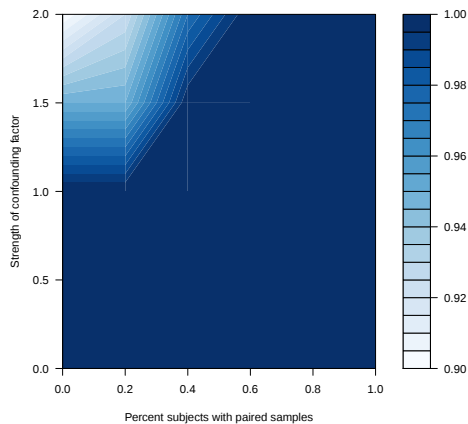
Median power with 200 total samples
