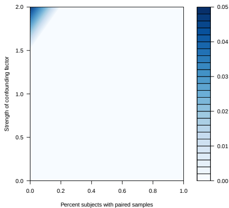
Range power with 500 total samples
