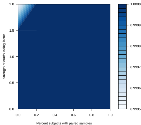
Ave. power with 500 total samples
