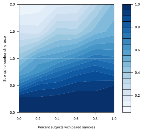
Ave. power with 50 total samples
