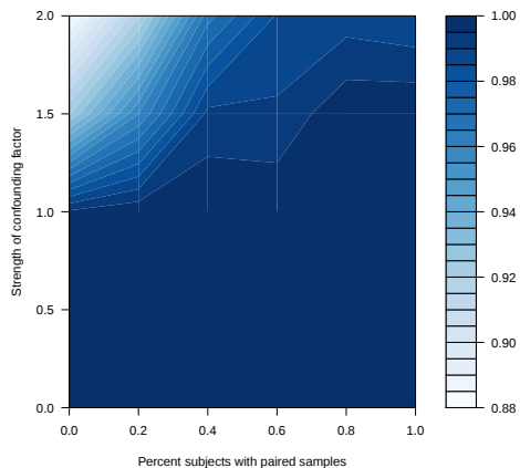
Ave. power with 200 total samples
