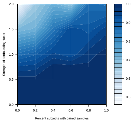
Ave. power with 100 total samples
