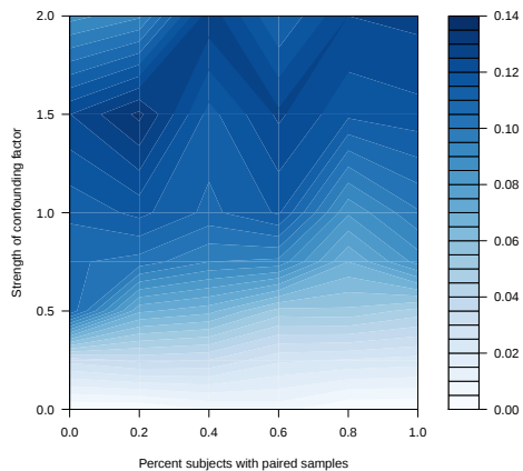
SD power with 50 total samples
