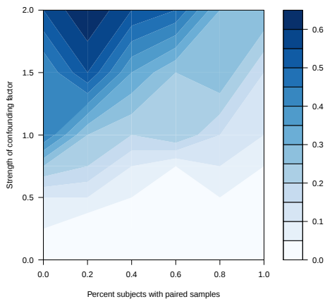
Range power with 100 total samples
