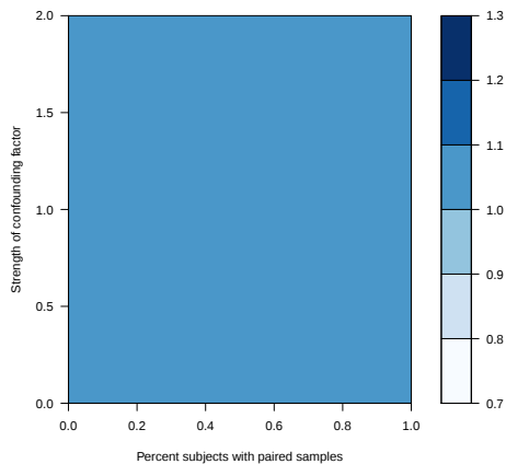
Median power with 500 total samples
