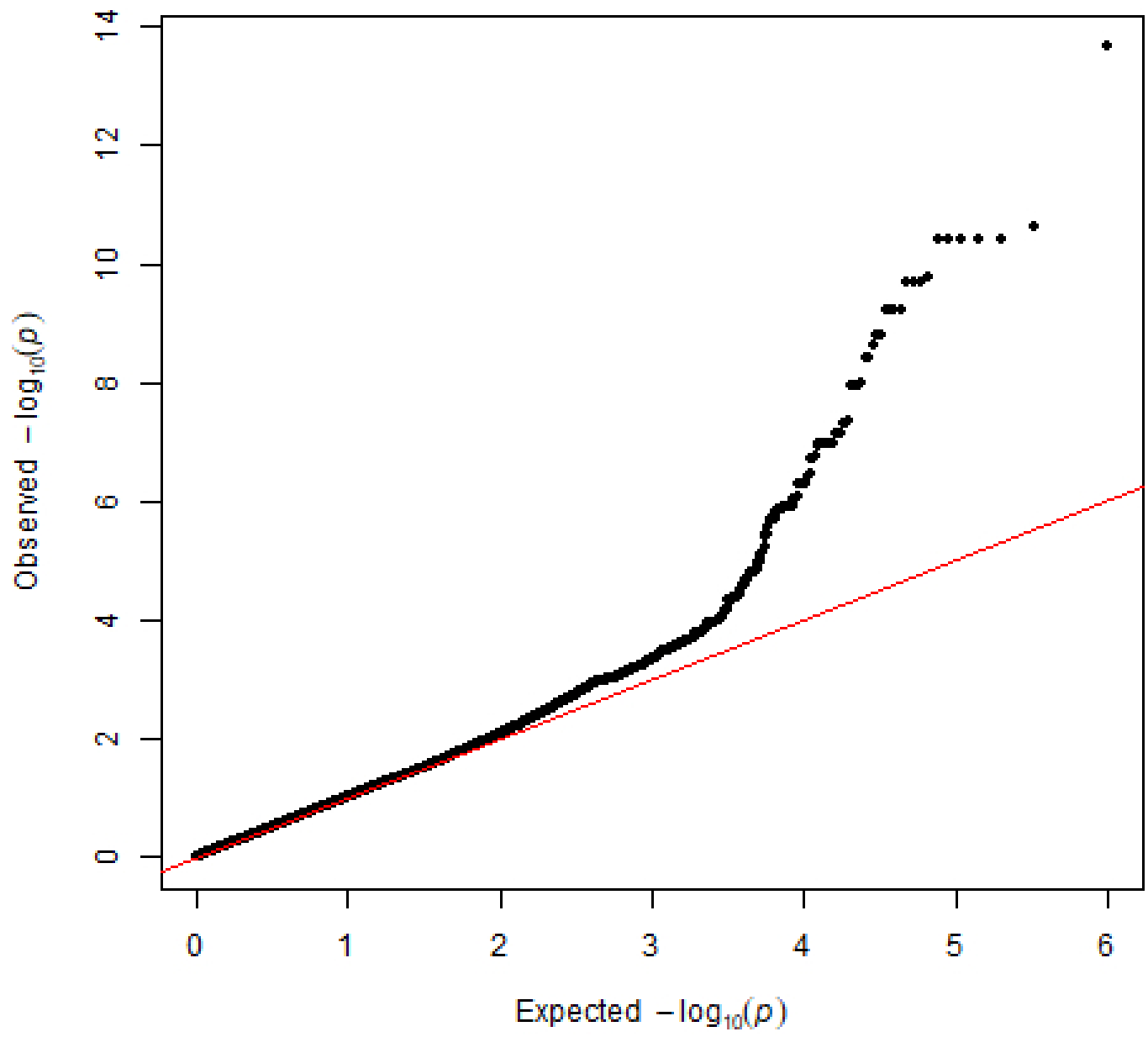
qqplot 3_2_0_0_0
