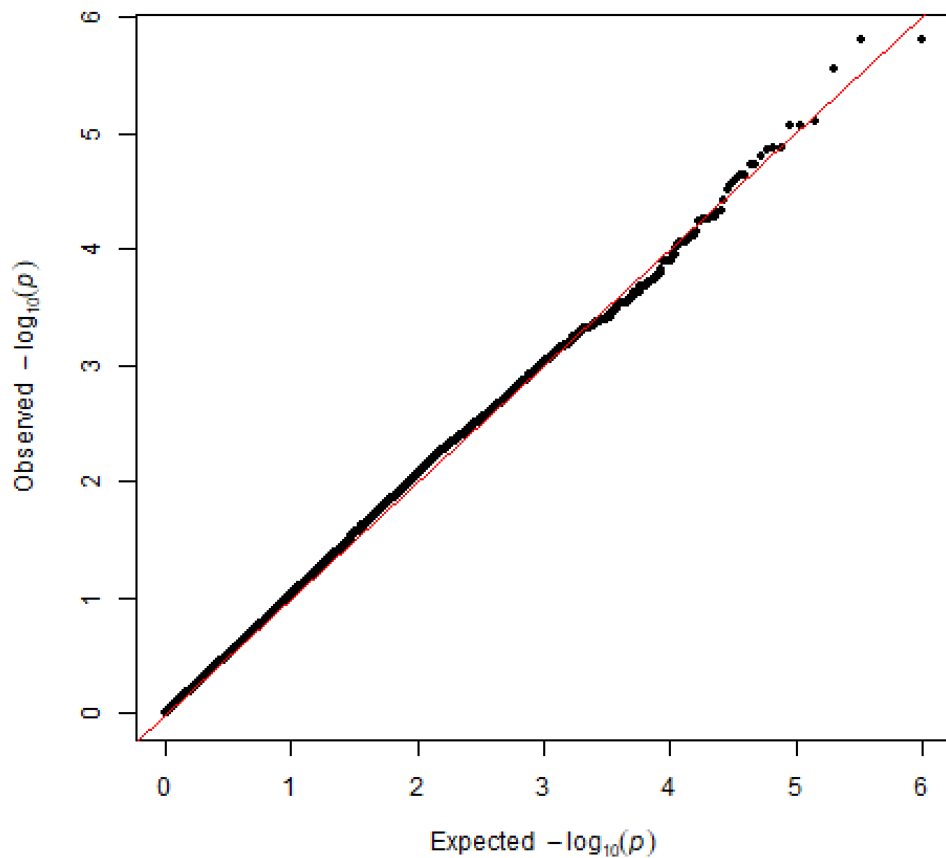
qqplot 2_0_0_1_0_6_sialyllactose
