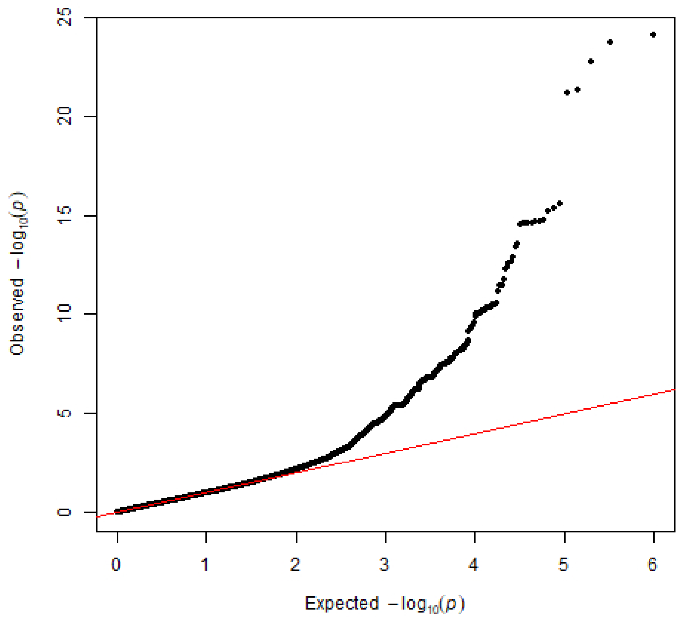
qqplot 5_4_1_0_0
