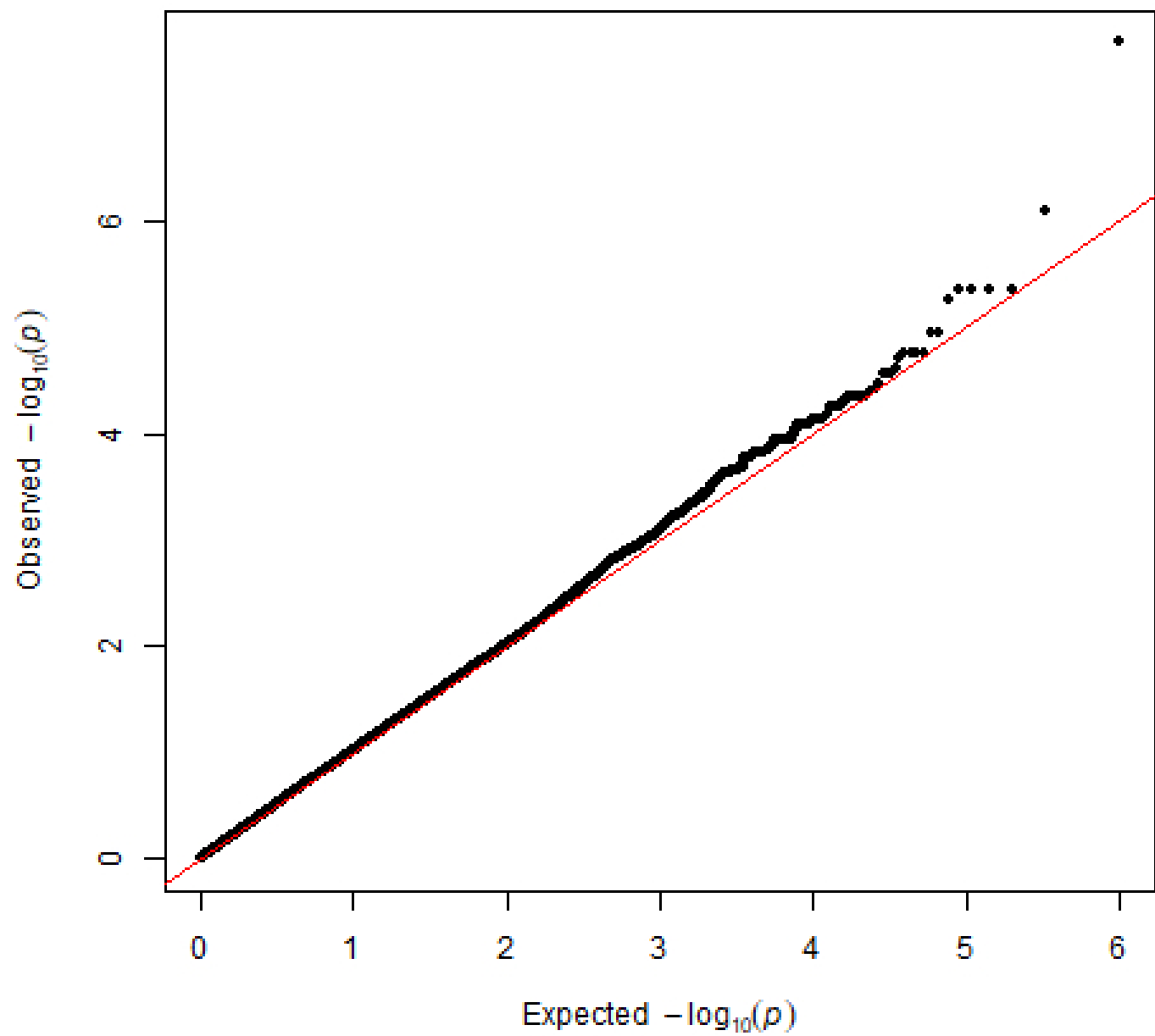
qqplot 2_0_0_2_0
