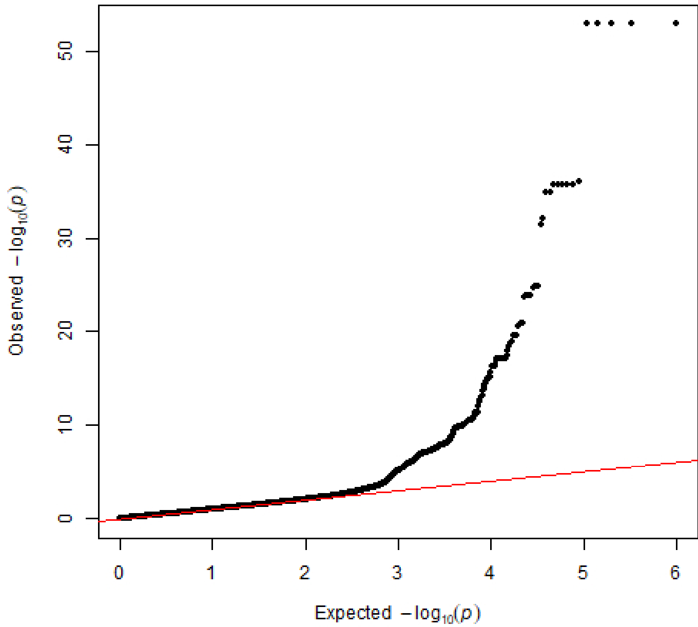
qqplot 2_1_0_0_0_isomer_1
