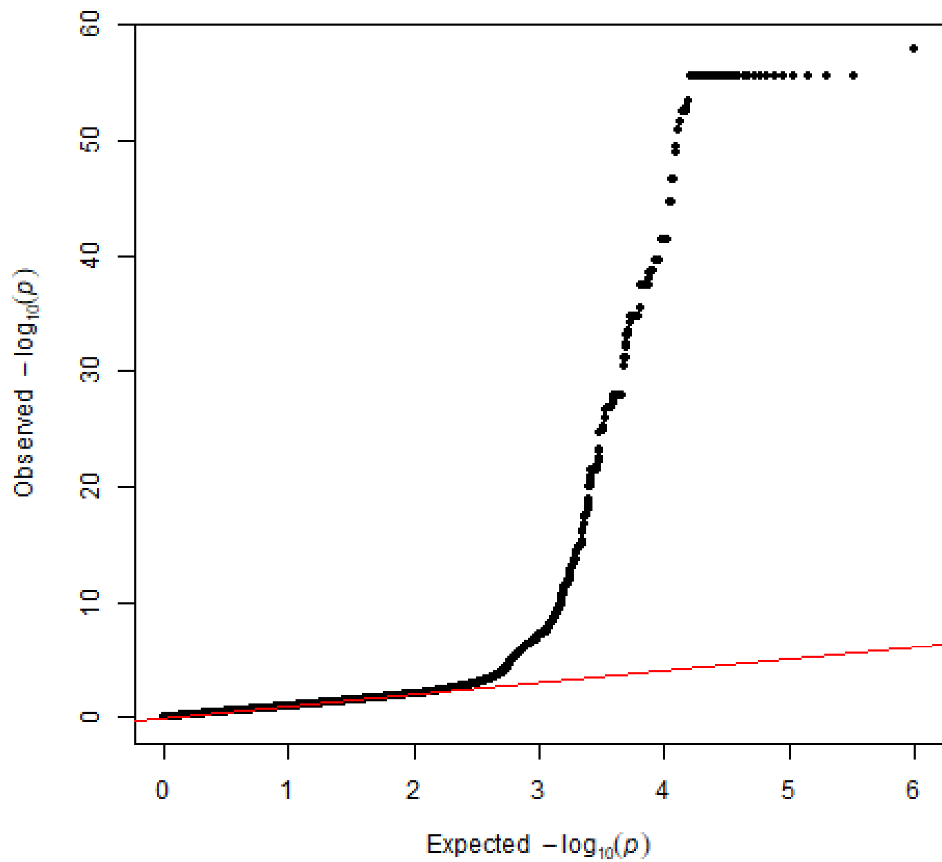
qqplot 3_1_0_0_0_Lacto_N_tetraose
