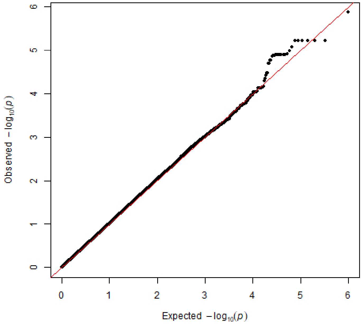
qqplot 3_1_0_0_0_isomer_2
