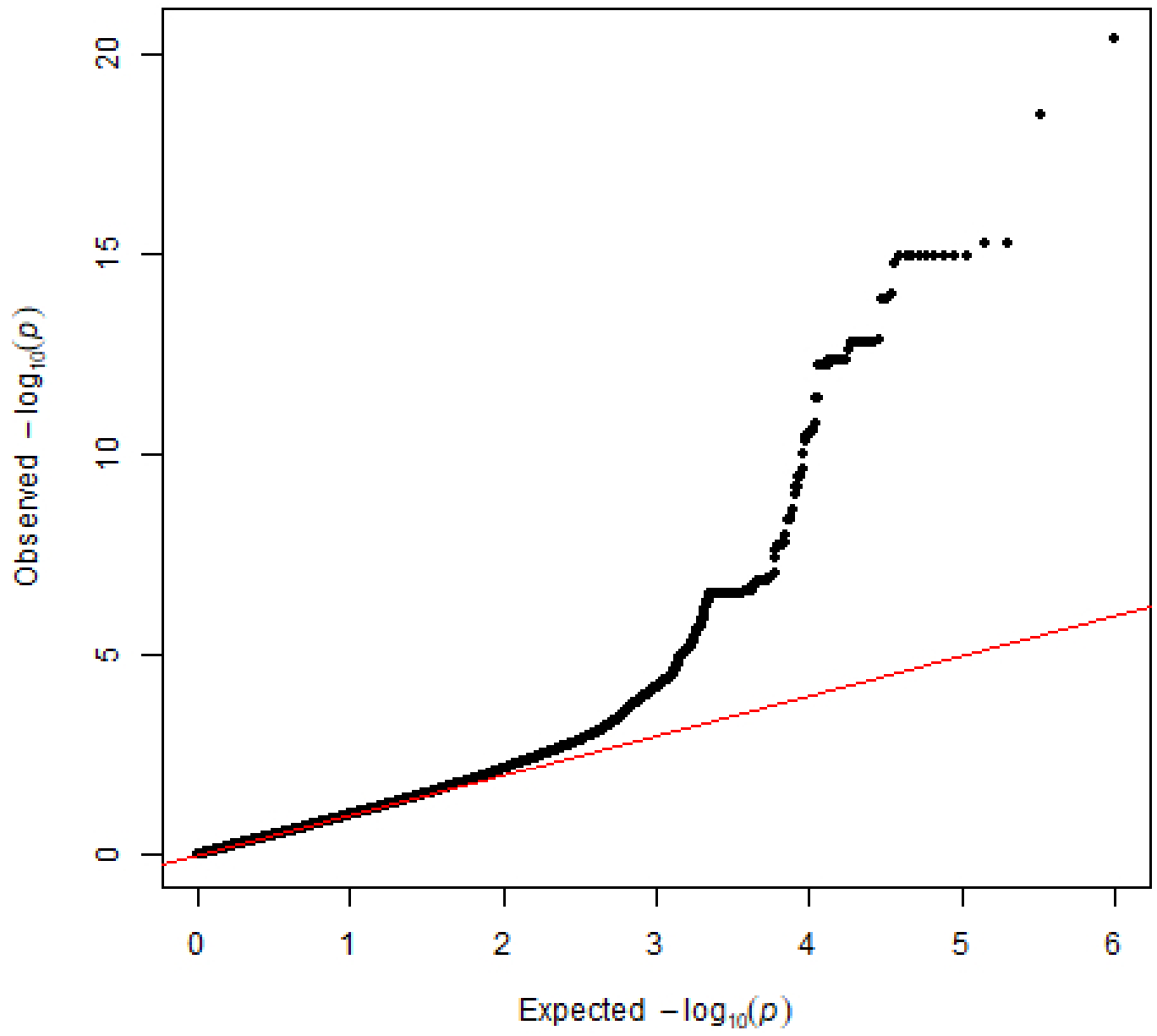
qqplot 4_1_0_0_0
