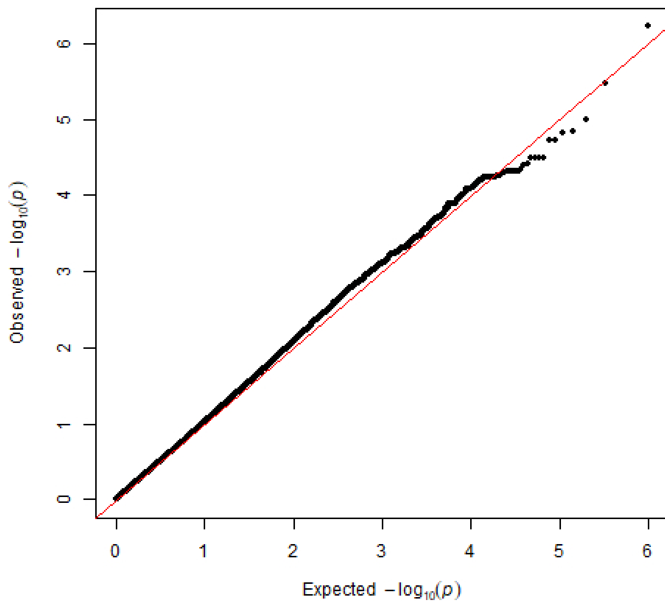
qqplot 2_0_0_1_0_3_sialyllactose
