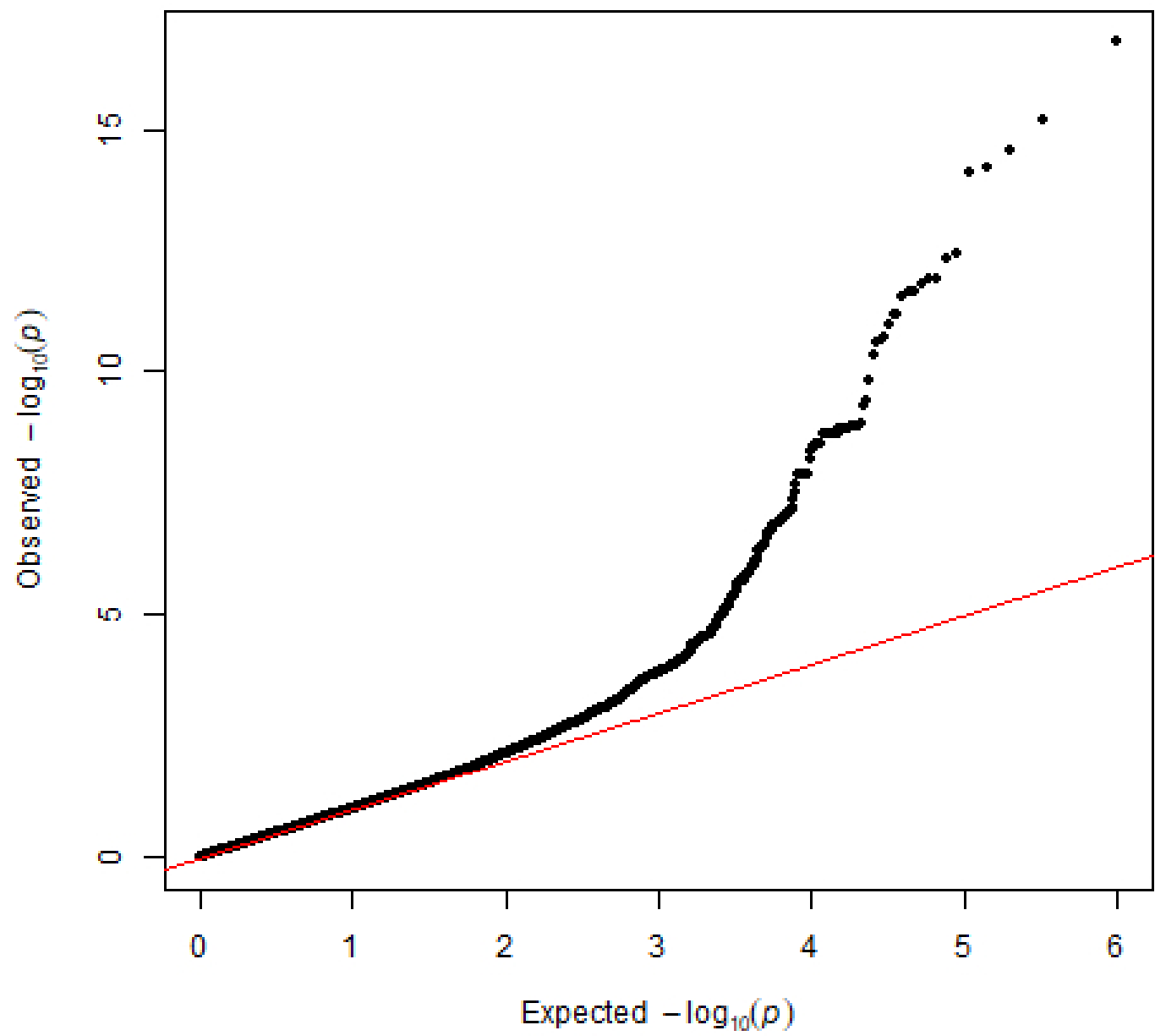
qqplot 4_4_1_0_0
