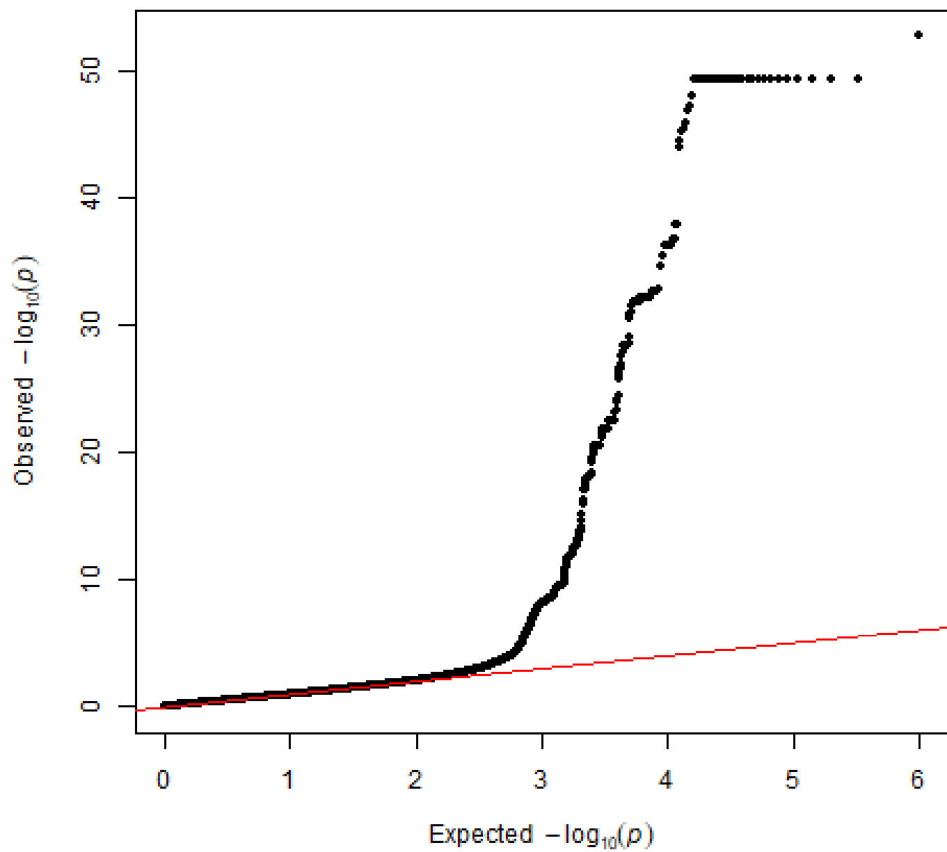
qqplot 4_2_0_0_0_Lacto_N_hexaose
