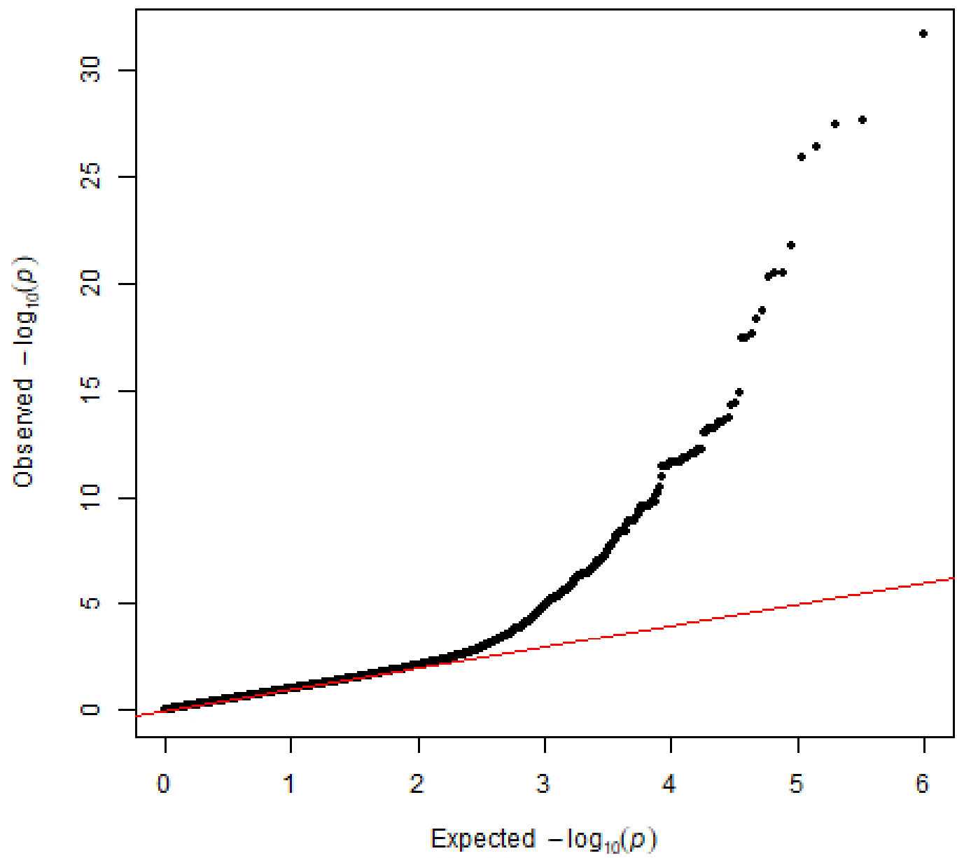
qqplot 3_6_1_0_0
