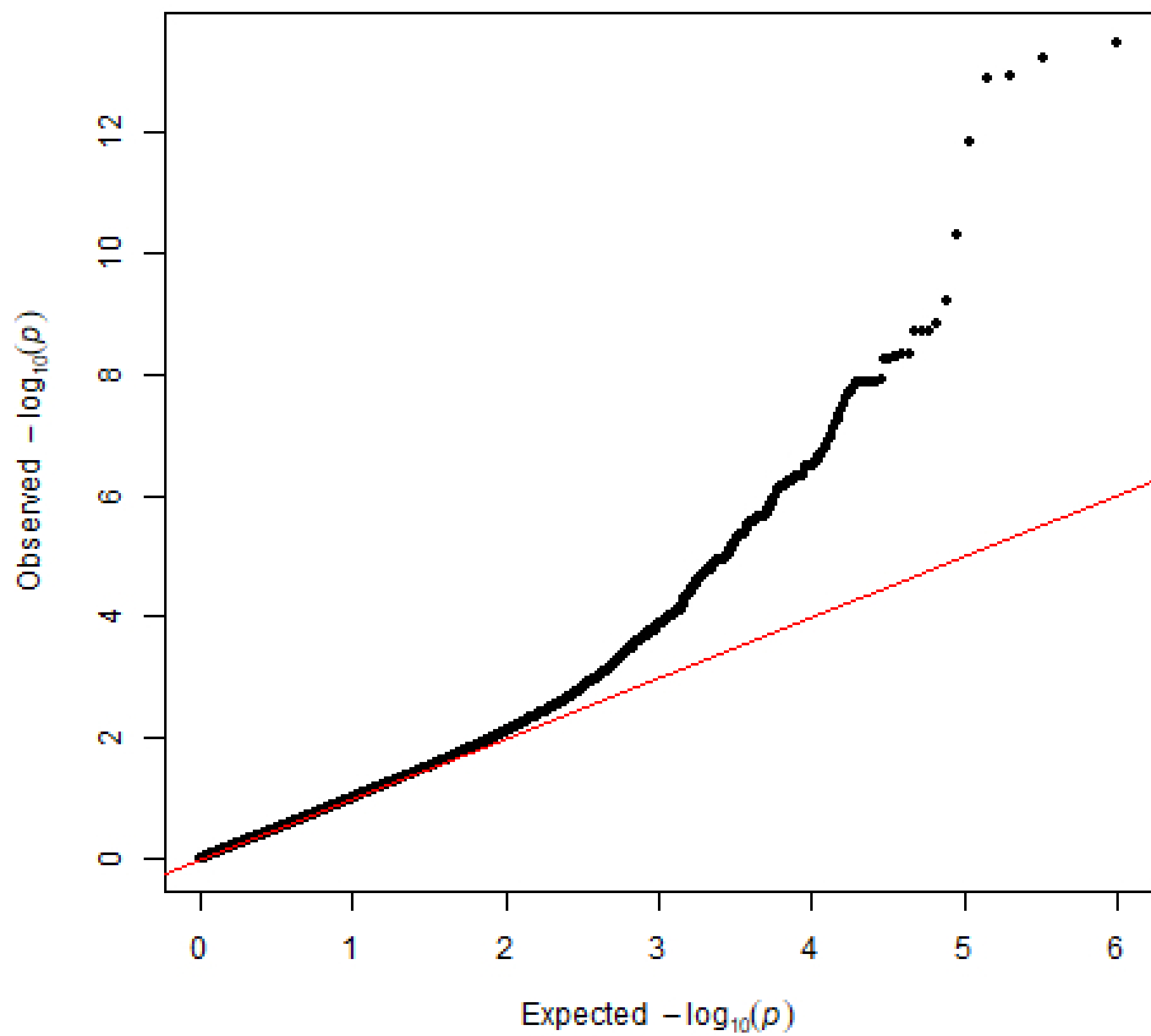
qqplot 5_4_0_0_0
