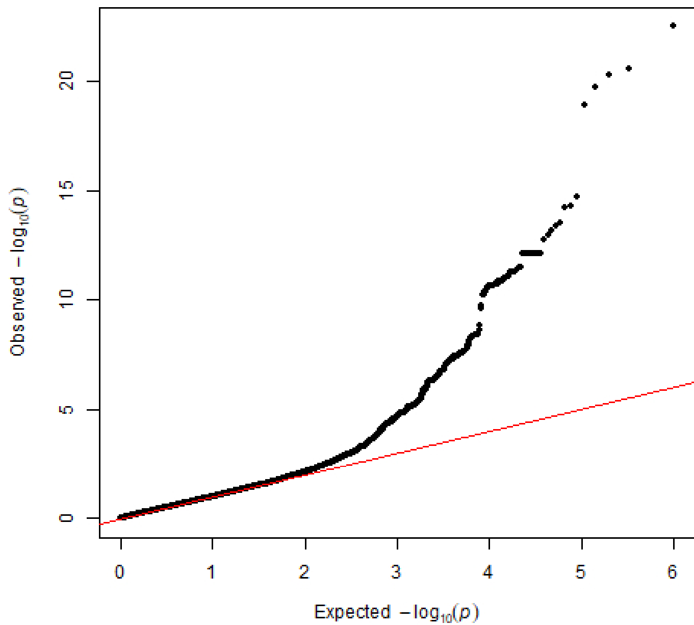
qqplot 4_5_1_0_0
