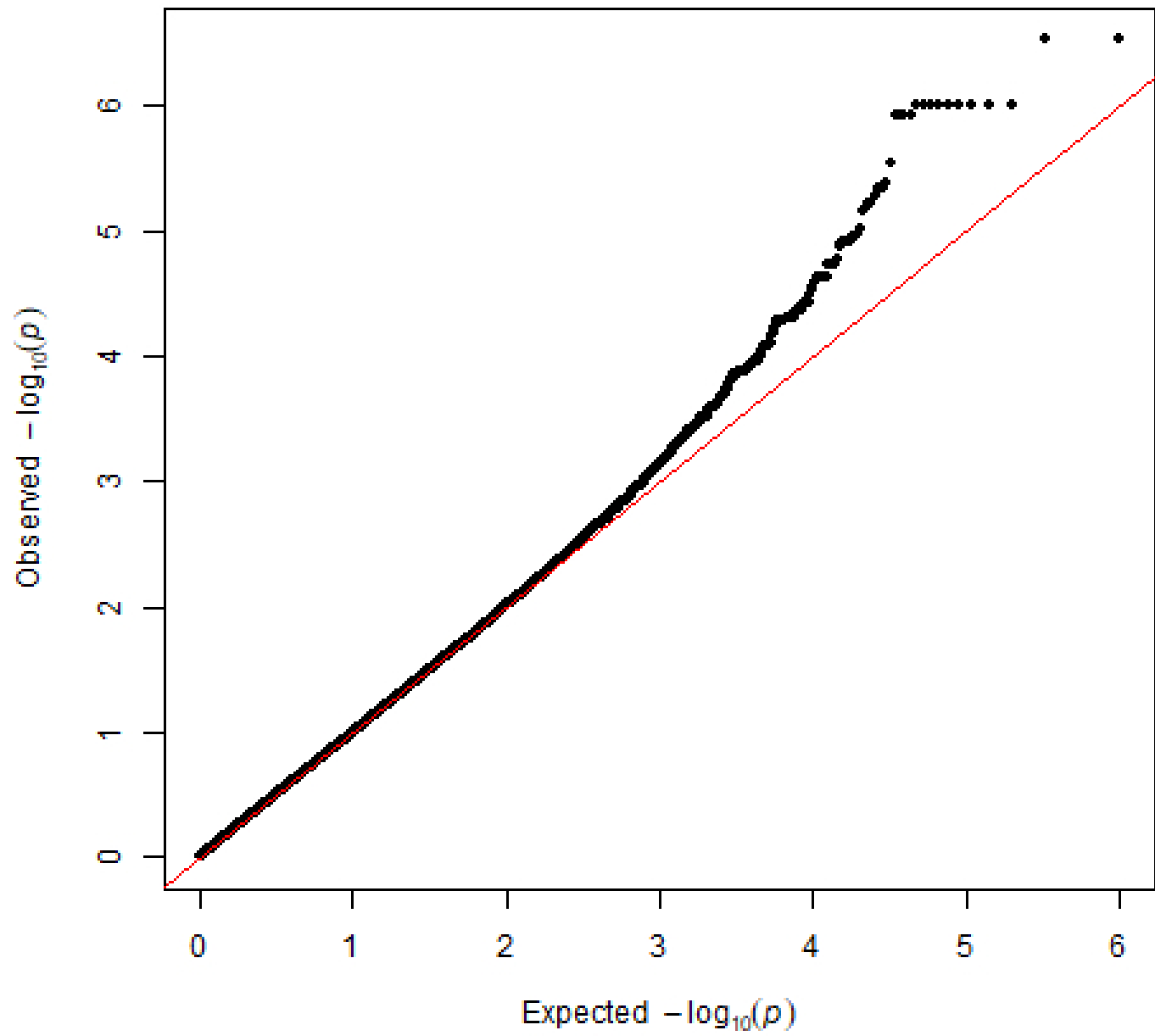
qqplot 2_1_0_0_0_isomer_2
