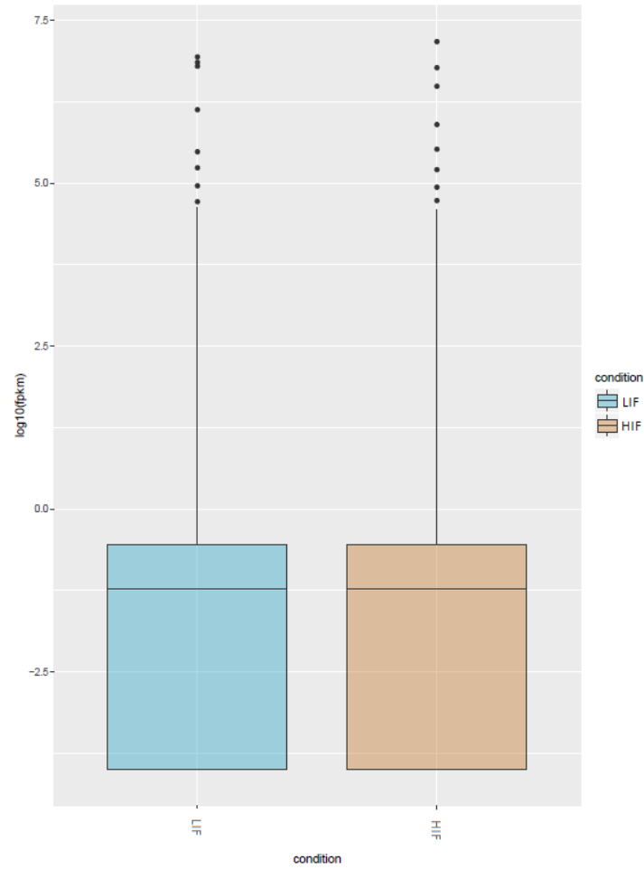
Additional Figure 1. Global statistics and quality control. (A) Box plot of FPKM distributions for individual conditions. (B) PCA plot for gene-level features.
