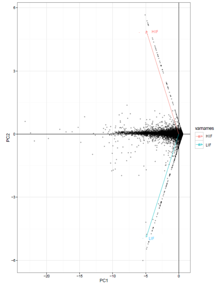
Additional Figure 1. Global statistics and quality control. (A) Box plot of FPKM distributions for individual conditions. (B) PCA plot for gene-level features.
