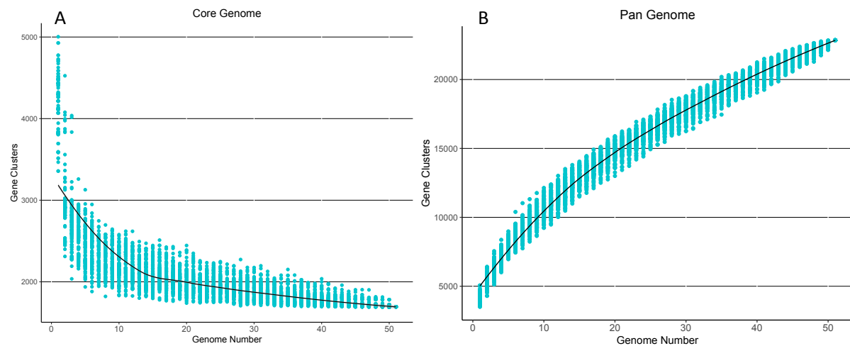
Supplementary Figure 3 Core and Pan-genome of 51 Vibrio isolates in this study. (A) The core-genome represents all genes shared by each genome added. (B) The pan-genome represents the accumulation of all genes among all genomes with each genome added.
