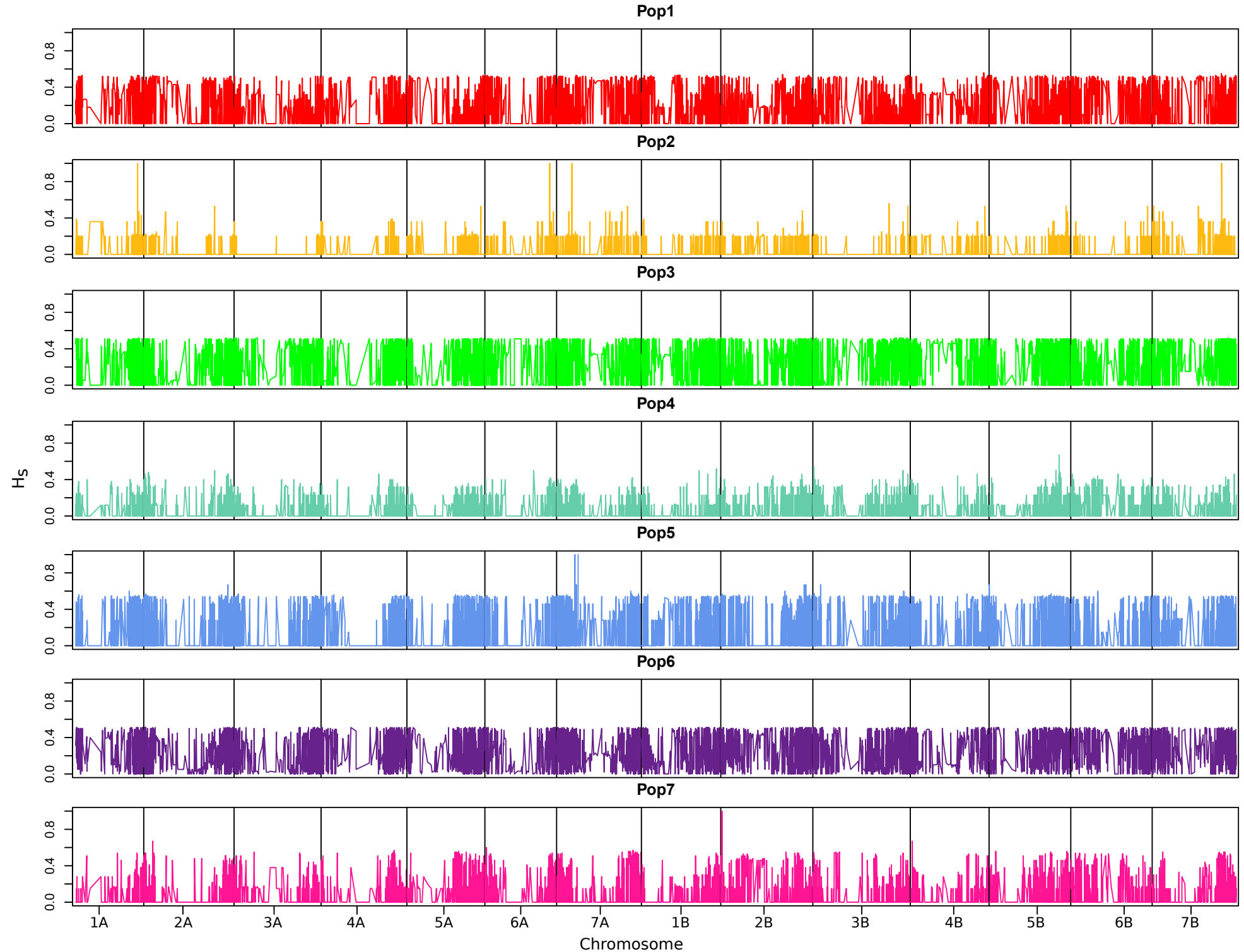
Additional file 6. Figure showing the genetic diversity ( H_s ) distribution across the A and B genomes in the different durum wheat populations identified with fastStructure.
