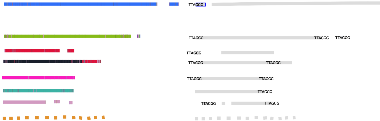
Flye assembly with Ratatosk corrected reads
