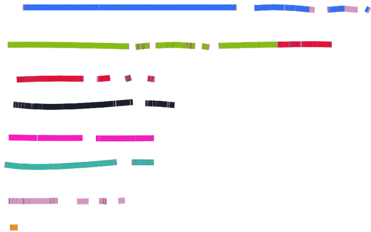
Raven uncorrected reads assembly
