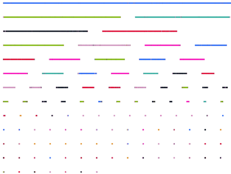
Canu uncorrected reads assembly
