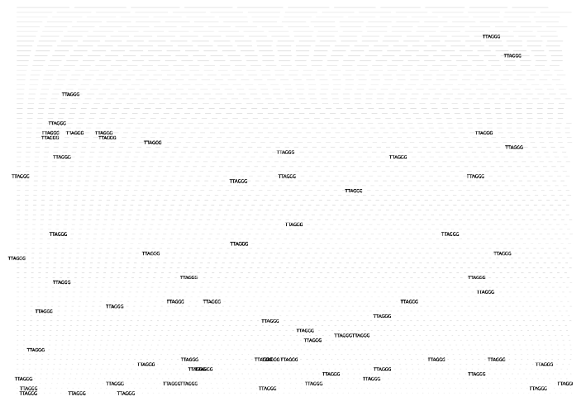
Canu assembly with FMLRC corrected reads
