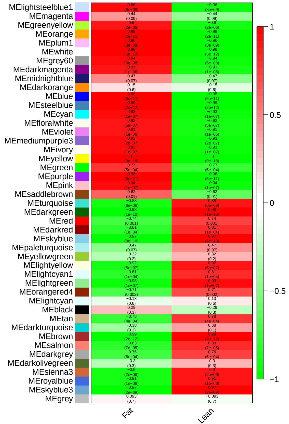
Module--trait relationships in GSE49121
