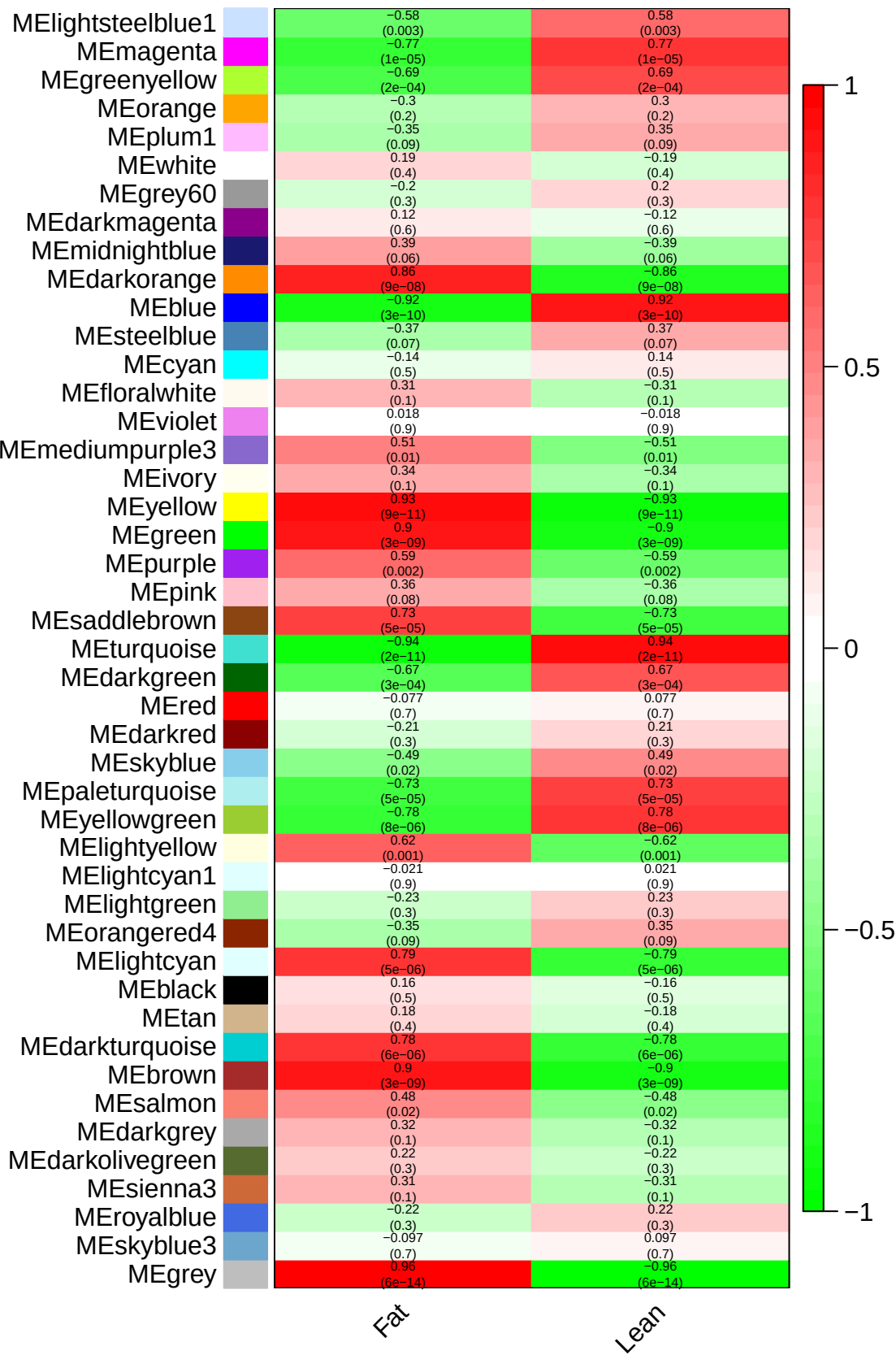
Module--trait relationships in GSE42980
