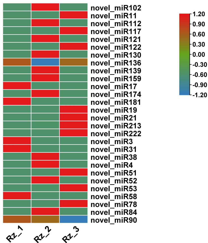
Supplementary Figure S3. Expression profiles of novel miRNAs during rhizome development. Rz_1: Rhizome 1st I_d; Rz_2: Rhizome 2nd I_d; Rz_3: Rhizome 3rd I_d.
