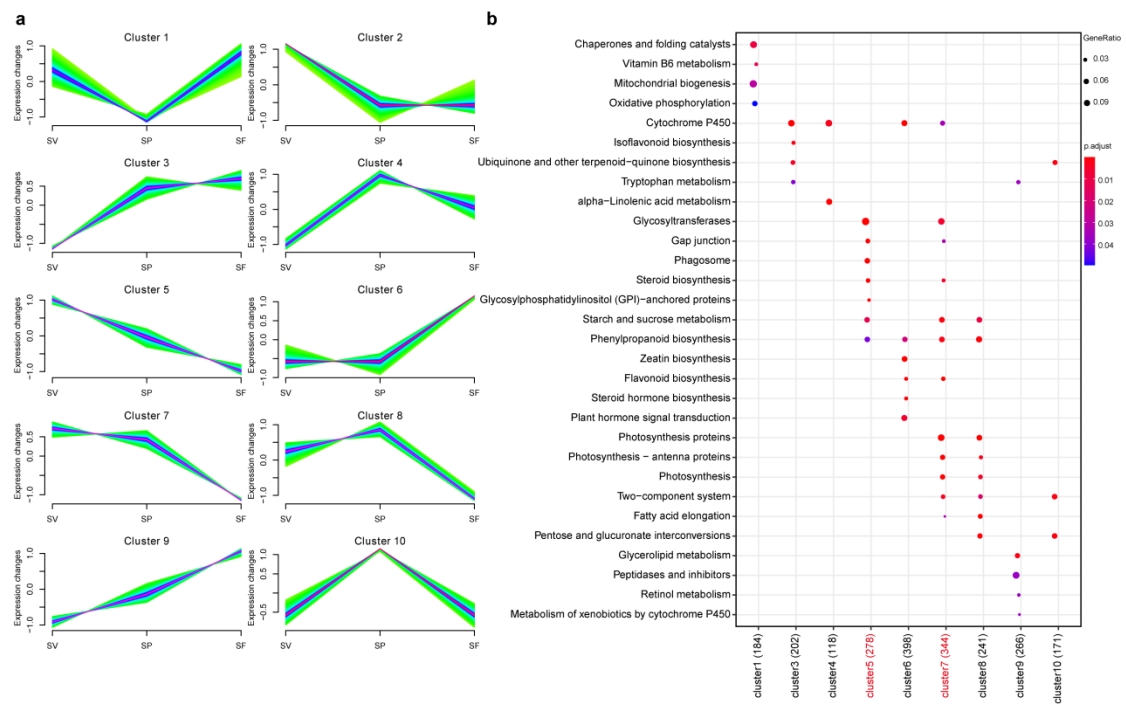
Figure S4 Ten cluster of DEGs in stem and the relative KEGG enrichments.
