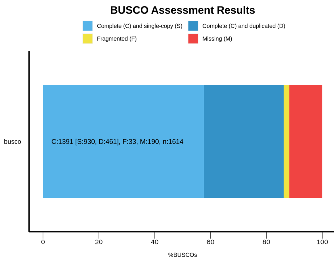
Figure S1 BUSCO assessment results.
