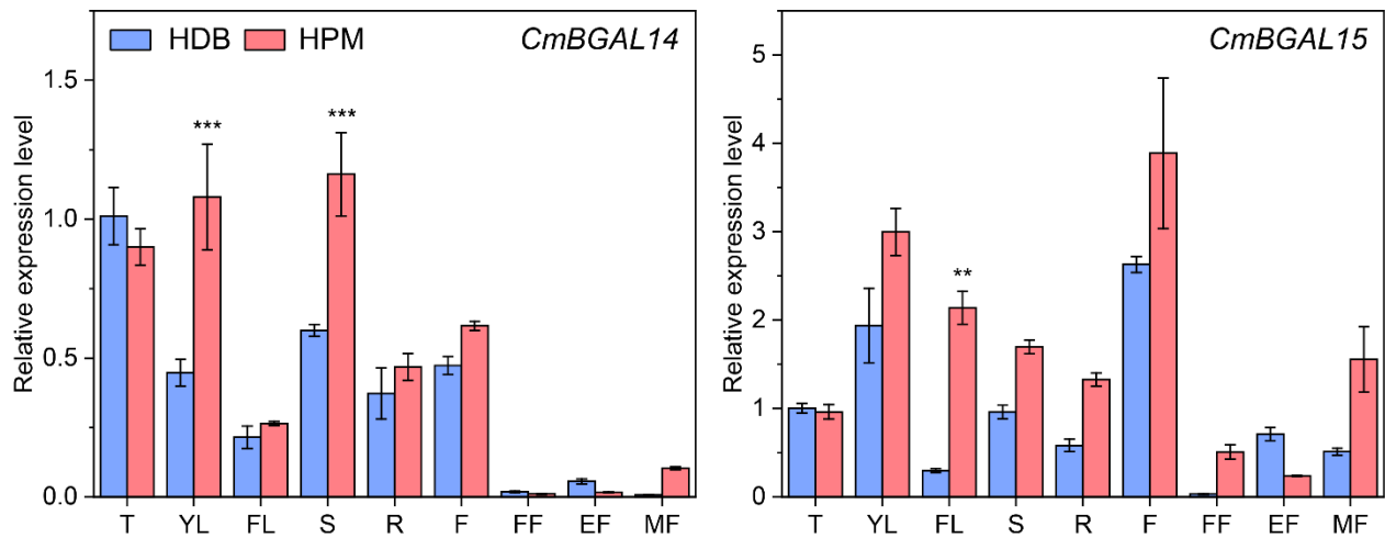
Additional file 4: Figure S4 Relative expression level of CmBGAL members in Clade E of ‘HDB’ and ‘HPM’ in various tissues. T: tendril; YL: young leaf; FL: functional leaf; S: stem R: root; F: flower; FF: fruitlet fruit; EF: expanding fruit; MF: mature fruit. The vertical bars indicate the standard error of the means of triplicates. Significant differences between the means were compared by Tukey test with * P < 0.05 , ** P < 0.01 and *** P < 0.001
