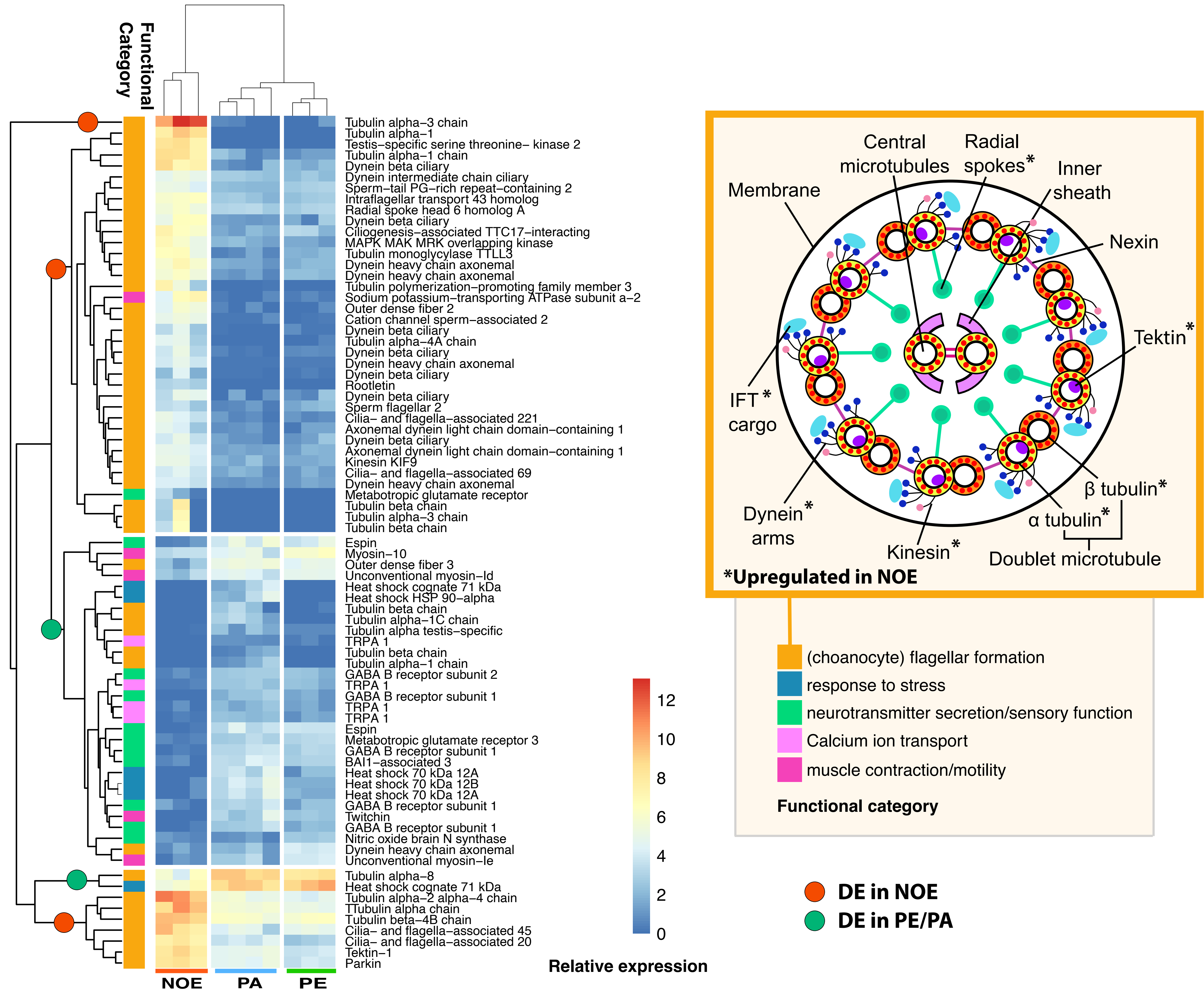
Supplementary Figure 4. Differentially expressed genes related to ciliogenesis, stress, contractility, and sensory functions. GO terms are shown on the left side with parent categories on the right. The detailed structure of the flagellum is shown on the right side of the figure.
