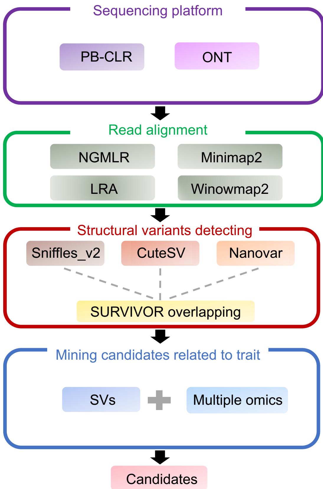
Additional file 8. The overall workflow for SV detection using three SV-calling programs on PB-CLR and ONT sequencing data.
