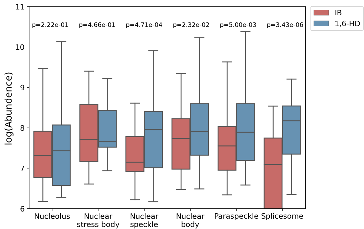
Figure S2. Biomolecular condensates in CHS-MS.
