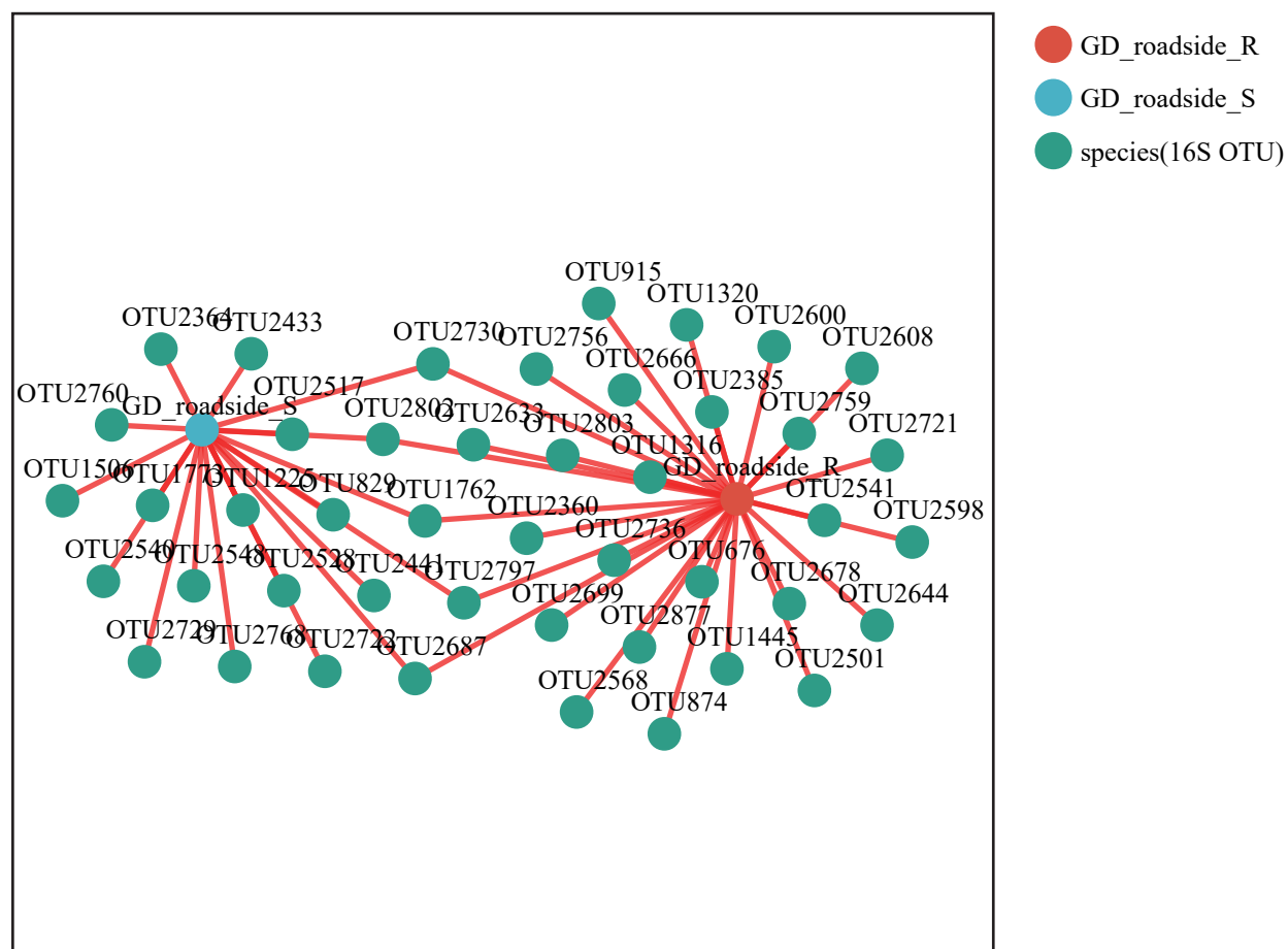
Supplementary Figure 5 Diagram of the co-occurrence network at the 16S OTU. A: in GA; B: in GD_understory; C: in GD_roadside; D: in GE. The network contains the species node and sample node, and their wires represent that the sample contains the species. GA, Geoderma attenuatum ; GD, Geodorum densiflorum ; GE, Geodorum eulophioides ; OTU, operational taxonomic unit.
