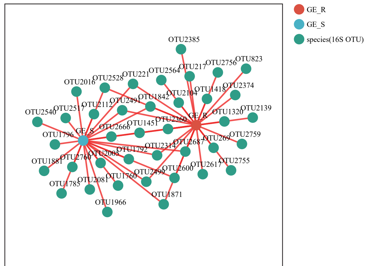
Supplementary Figure 5 Diagram of the co-occurrence network at the 16S OTU. A: in GA; B: in GD_understory; C: in GD_roadside; D: in GE. The network contains the species node and sample node, and their wires represent that the sample contains the species. GA, Geoderma attenuatum ; GD, Geodorum densiflorum ; GE, Geodorum eulophioides ; OTU, operational taxonomic unit.
