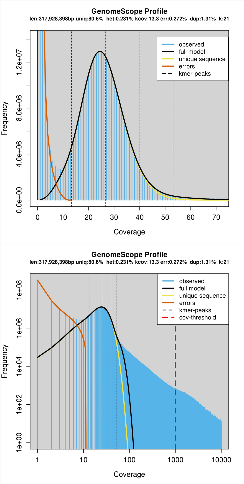
Fig. S7 GenomeScope profile plots of absolute (top graph) and log-transformed (bottom graph) k-mer frequency distributions, at a k-mer length of 21, built based on the SR1 reads.
