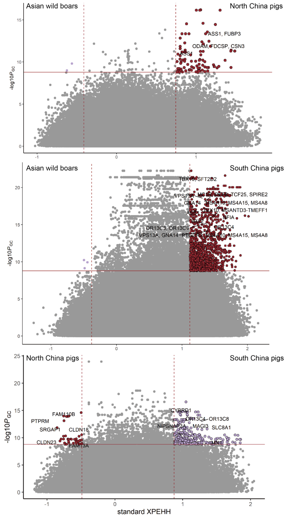
Figure S3. Overview / Distribution of the significant selection signatures in South and North China indigenous pigs. The x-axis and y-axis represent the standard XPEHH value and -\log_{10}P_{GC} .
