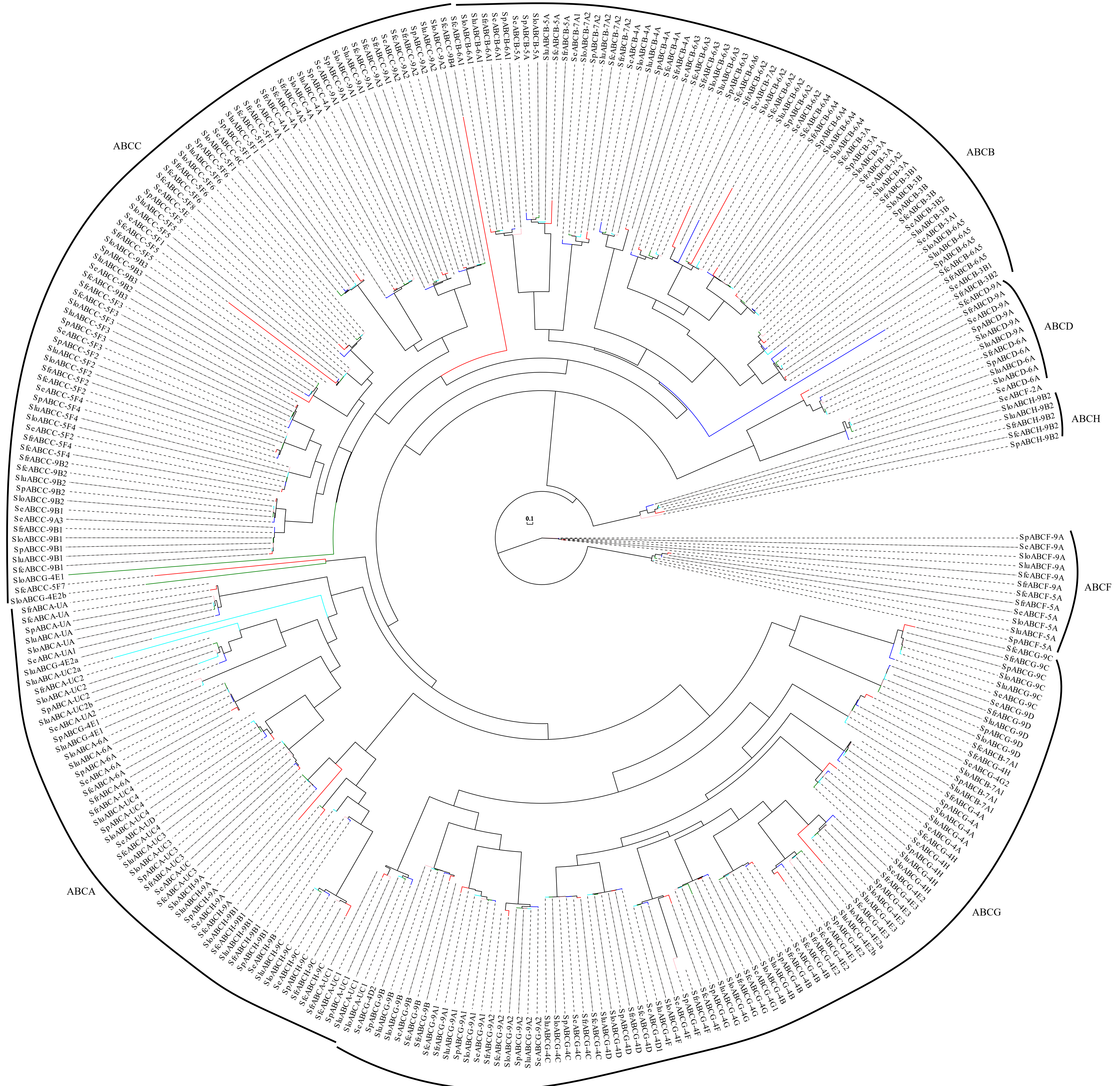
Supplementary Material 6: Fig. S6. Phylogenetic tree of phase III detoxification enzymes (ABC) of the genus Spodoptera constructed using ML
