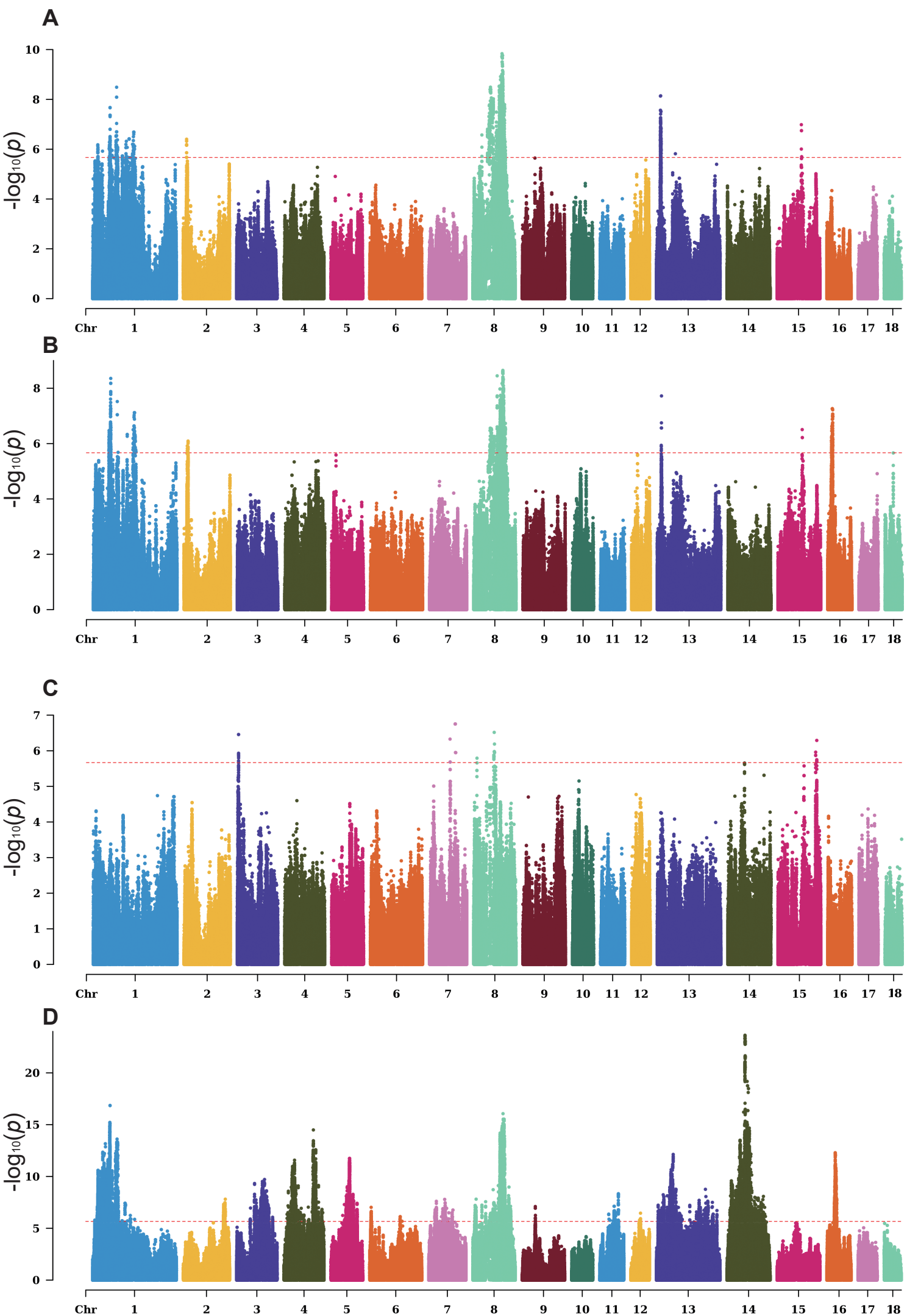
Figure S1 Manhattan plot showing GWAS results for reproduction traits in Yorkshire pigs. Traits included are TNB (A), NBA (B), WeightCV (C), and MLW (D). Significance threshold is indicated by the horizontal dashed line.
