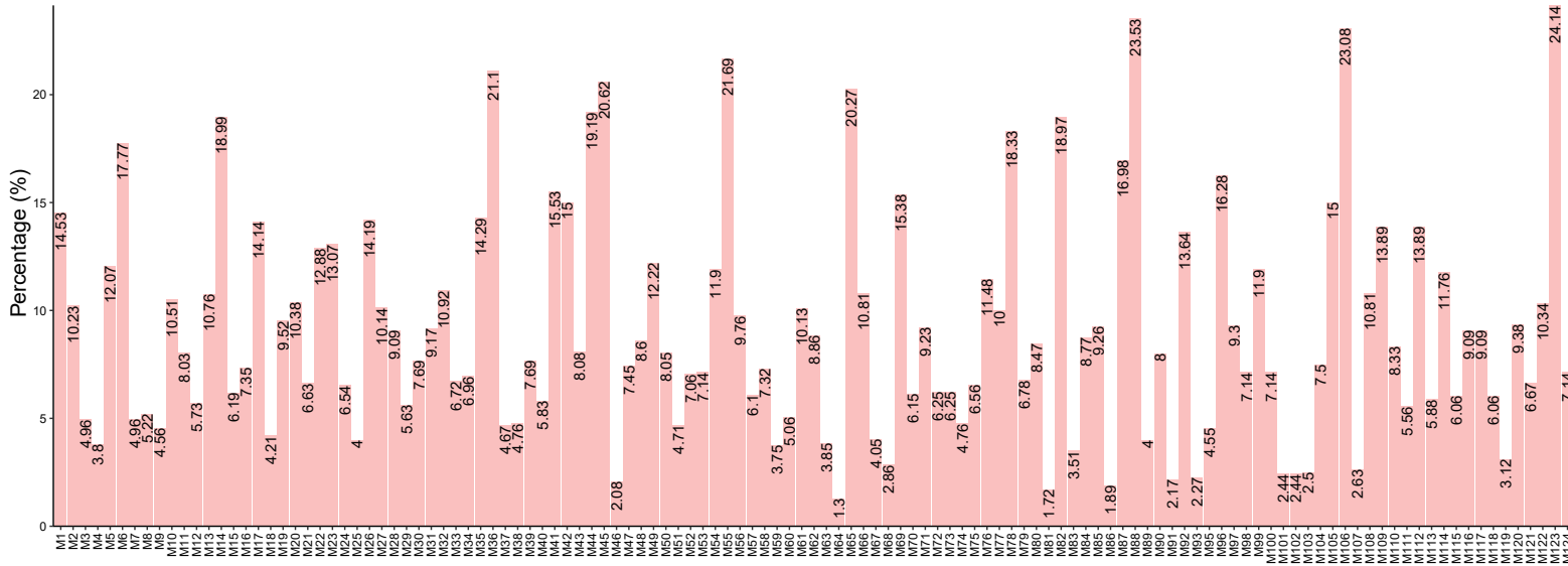
Figure S7. Proportion of TF genes within each module.
